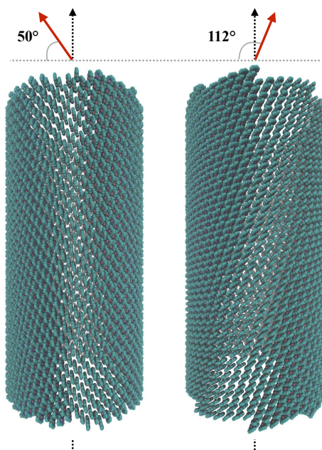
Figure A.3: Snapshots of pre-assembled helical tubes: \delta = 50^\circ (left) and \delta = 112^\circ . For clarity, side groups of the head part and tails are not shown. The \mathbf{a} packing vectors are shown by red arrows.
