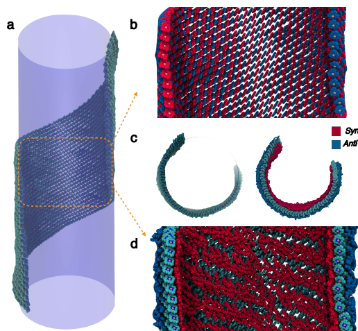
Figure 2.5: Details of the syn-anti packing for the curved structure obtained after 1 ns MD simulation of (30, 30) BChl c system at 50 K. Syn and anti BChl c molecules are shown in red and blue respectively. (a) Curved structure (repeated from Figure A.12a) and fitted cylinder. For clarity, side groups of head part and tails are not shown; (b) syn-anti packing of heads, showing high order of head parts even in curved domain; (c) Projection of the pigment assembly along the cylinder axis with and without tails, displaying the spatial extent of the tails in the curved structure. The concave (convex) side of the curved structure is covered by syn ( anti ) tails, respectively; (d) Details of the tail structure, illustrating the groove like nature of the tail phase at the concave side of the curved structure, leaving enough free space for other molecules to occupy, as well as the liquid-crystal like order of the tail phase for this low temperature.
