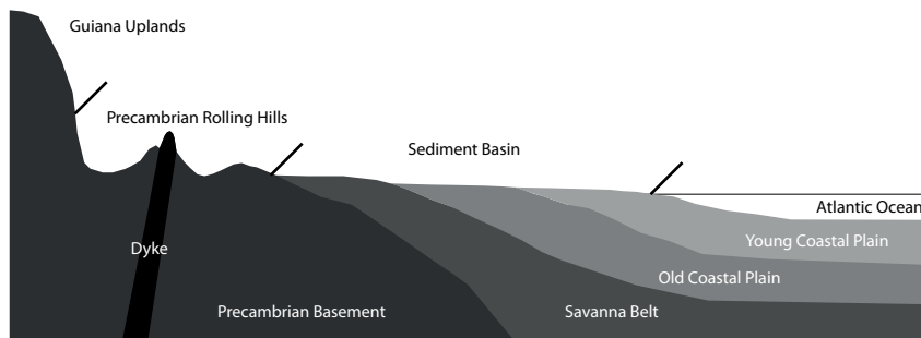
Fig. 2.3: Simplified north-south section of Guiana (adapted from Noordam 1993:15; Krook 1984).
