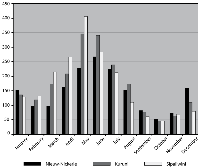
Fig. 2.6: Weather station's annual averages on the Corentyne (data adapted from Nurmohamed 2008: 67-8).
