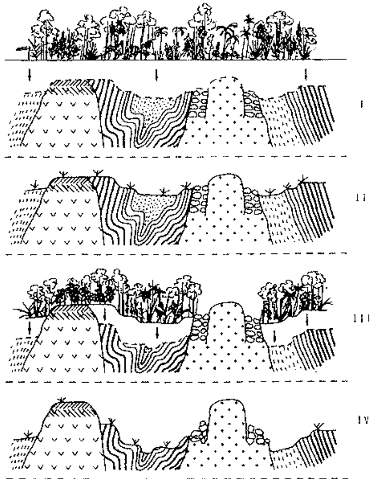
Fig. 2.4: The development of erosion and weathering of the undulating granitoid landscape (Kroonenberg & Melitz 1983:398), reprinted with permission of the first author.
