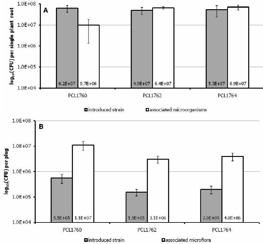
Fig. 5. Colonization of the tomato root (Panel A) and of the stonewool substrate (Panel B) by P. putida strain PCL1760 and its mutants PCL1762 ( dctA ) and PCL1764 ( flhA ) at the end of a biocontrol experiment.
