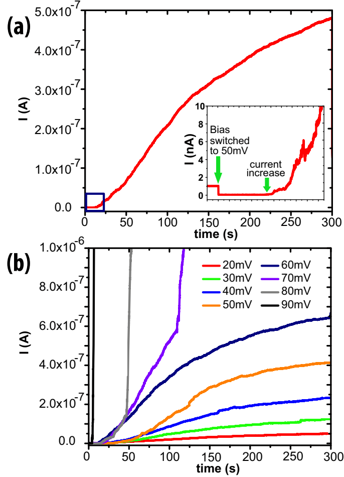
Figure 5.3: a) Current evolution observed when a step in the voltage from -1V to +50mV is applied to the sample. The inset shows the first seconds of the trace. b) Traces measured at bias voltages from +20mV up to +90mV
