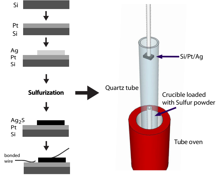
Figure 2.1: Schematic diagram of the fabrication steps of the \text{Ag}_2\text{S} devices and drawing of the oven set up used to sulfurize the Ag thin films.
