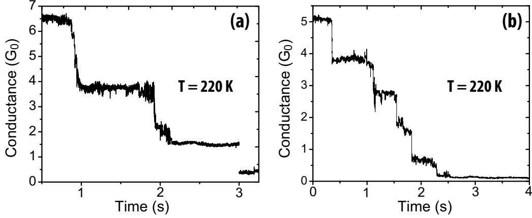
Figure 6.4: Steps in the conductance observed at 220K when breaking the conductive path at a bias of -100 mV. The breaking traces show clear conductance steps of approximately 1G_0 at the last stages of breaking.
