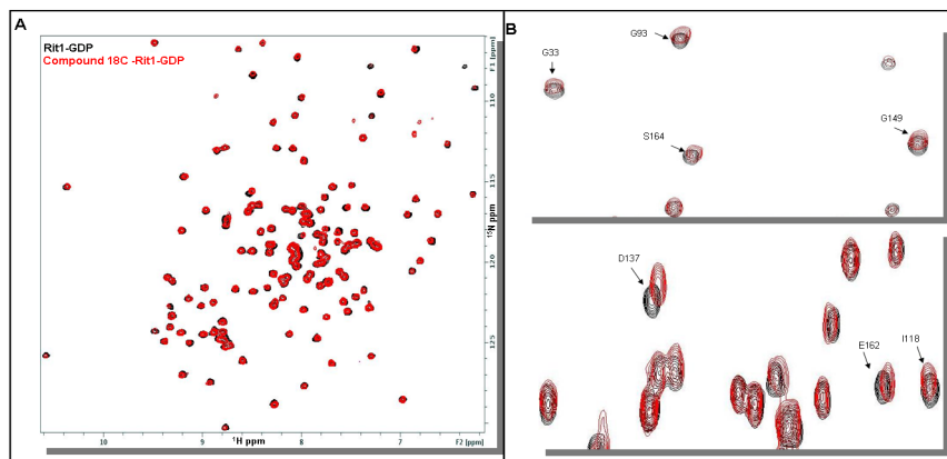
Figure S9. A] The overlay of the ^1\text{H} , ^{15}\text{N} HSQC spectra of Rit1-GDP (black) and in the presence of 1mM compound 18c (red). B] The zoomed region of the overlaid ^1\text{H} , ^{15}\text{N} HSQC NMR spectra shown in (A). The residues that show significant CSPs are labeled.
