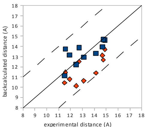
Figure S7. Comparison of back calculated and observed distances averaged over top 10 structures with error limits of \pm 3 Å shown by dashed lines. Solid line represents the perfect correlation. The blue squares indicate the lowest docking solutions obtained by treating the intermolecular restraints as two separate sets. The red diamonds shows the distances obtained by simulation consisting of all inter-molecular PRE distance restraints in one set. As only two PRE restraints were available for the acidic moiety of 18c , the force constant for PREs was increased from 3.0 to 90.0 to get a significant energy penalty whenever the PRE restraints were not fulfilled.
