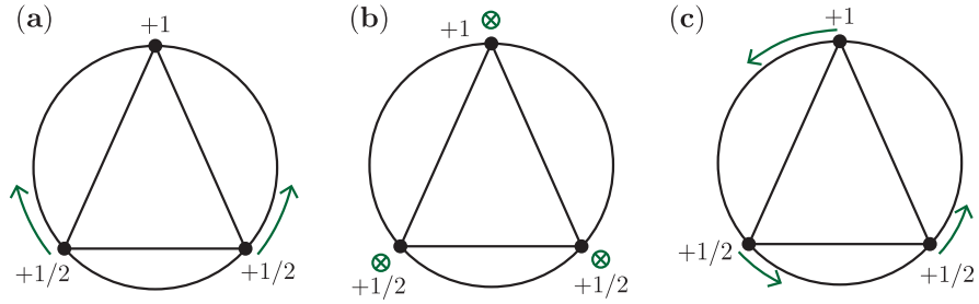
Figure 20: Schematics of the three non-trivial eigenmodes corresponding to (a) \mathbf{u}_4 , (b) \mathbf{u}_5 and (c) \mathbf{u}_6 . The defects (represented by dots) continue to lie on a great circle in (a) and (c), but not in (b). The defects continue to form an isosceles triangle in (a) and (b), but not in (c).
