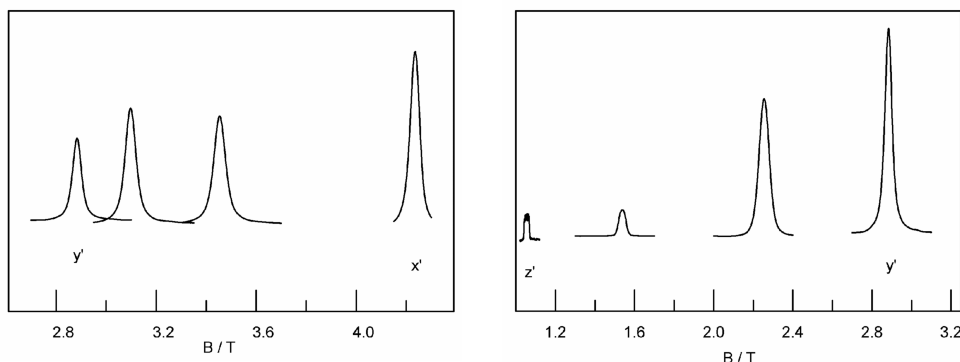
Figure 4.2: W-Band ESE-detected EPR spectra of a crystal of 1% Co iPr,Ph L 2 /Zn iPr,Ph L 2 at different orientations of the magnetic field with respect to the crystal. The spectra in the upper figure correspond to orientations in the x'y' plane, in the lower figure in the z'y' plane. At z' the cobalt hyperfine splitting of the line is resolved.
