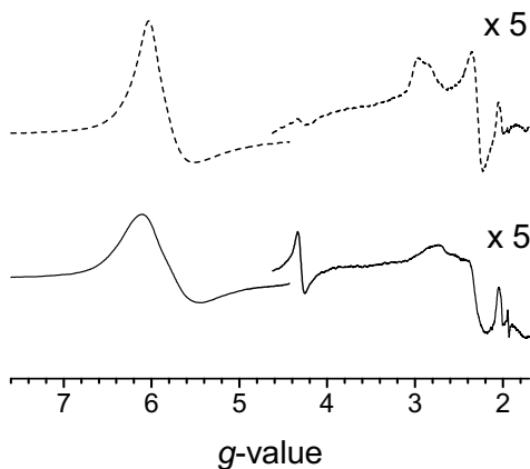
Figure 6.8. X-band EPR spectra of u-cytc550 (dashed line) and u-cytc550 after addition of 3 equivalents \text{H}_2\text{O}_2 (solid line). The samples contained approximately 1 mM protein and were in 30% glycerol, 4.2 M Gdn.HCl, 70 mM sodium phosphate. The sample of u-cytc550 and that after addition of 3 equivalents \text{H}_2\text{O}_2 were at pH 5.3 and 5.4, respectively. The positive signal at g = 2.04 is an artefact of the resonator.
