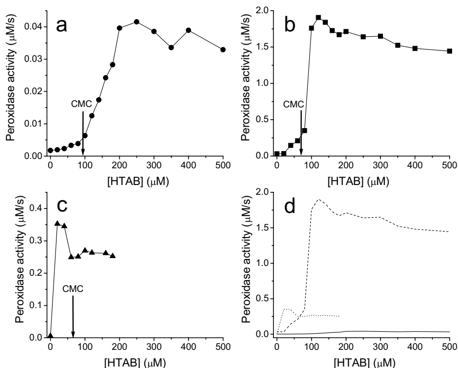
Figure 5.5. Peroxidase activity of cytc550 as a function of total added HTAB at pH 4 (a), pH 8 (b) and pH 11 (c). In all cases [cytc550] was 0.61 \mu\text{M} , [gc] was 10 mM, [ \text{H}_2\text{O}_2 ] between 0.6 and 30 mM, and [phosphate] was 100 mM. Arrows indicate the CMC of HTAB determined for each pH value. In d), the activity increase at pH 4 (solid line), pH 8 (dashed line) and pH 11 (dotted line) is reproduced for direct comparison of the respective activities.
