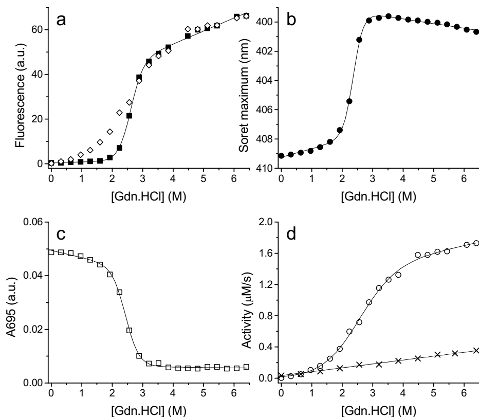
Figure 4.2. Equilibrium unfolding of horse heart cytc by Gdn.HCl at pH 4.5 (298 K) followed by a) tryptophan fluorescence increase (■), b) Soret band shift, c) 695-nm absorbance decrease and d) peroxidase activity increase (○). In a) the peroxidase activity increase is also shown (◇), and included in d) is the peroxidase activity of MP-8 as a function of [Gdn.HCl] (×). The protein unfolding data were fit to the two-state model of unfolding. [213] See Materials and Methods for details. [Cyt c] was 3.2 μM in the fluorescence and Soret measurements, and 60 μM in the 695 nm absorbance measurements.
