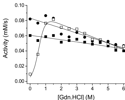
Figure 4.7. The peroxidase activity at pH 3.0 (298 K) of horse heart cytc (■), yeast iso-1-cytc (●) and P. versutus cytc550 (□) as a function of [Gdn.HCl]. The lines through the data points are drawn for reasons of clarity only.
