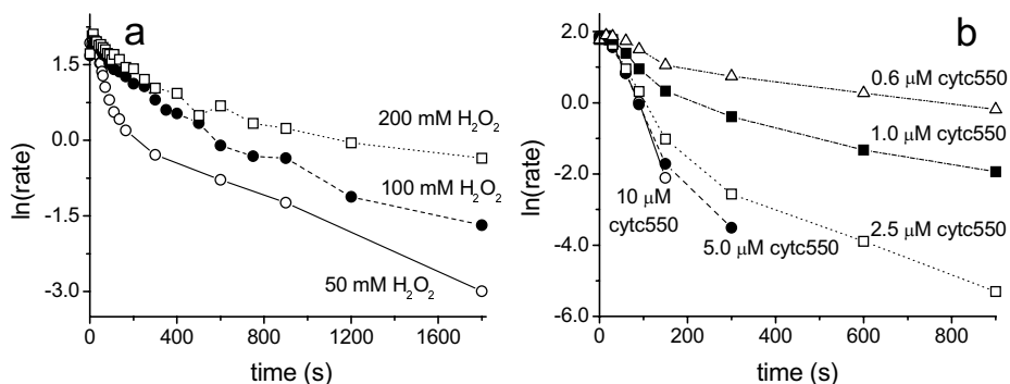
Figure 2.8. Rate of the steady-state peroxidase reaction as function of the pre-incubation time with \text{H}_2\text{O}_2 . In a ), [\text{cytc550}] was 1\ \mu\text{M} in the pre-incubation mix and [\text{H}_2\text{O}_2] was varied ( \circ , 50\ \text{mM} ; \bullet , 100\ \text{mM} ; \square , 200\ \text{mM} ). In b ), [\text{H}_2\text{O}_2] was 50\ \text{mM} in the pre-incubation mix and [\text{cytc550}] was varied ( \circ , 10\ \mu\text{M} ; \bullet , 5\ \mu\text{M} ; \square , 2.5\ \mu\text{M} ; \blacksquare , 1\ \mu\text{M} ; \triangle , 0.6\ \mu\text{M} ). Activity was assayed in 10\ \text{mM gc} , 50\ \text{mM H}_2\text{O}_2 , and < 0.5\ \mu\text{M cytc550} .
