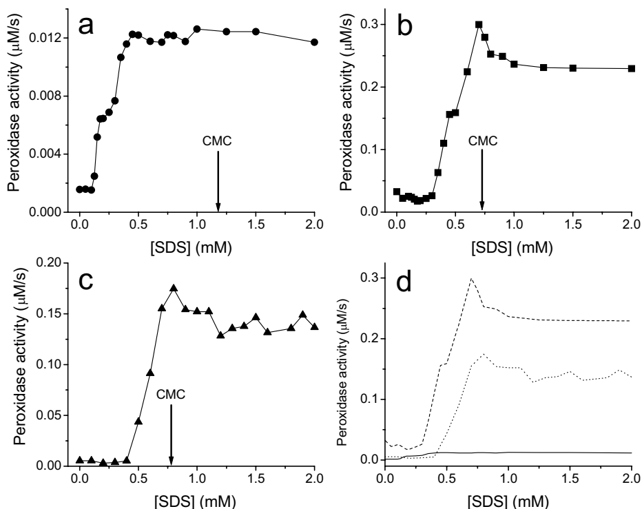
Figure 5.4. Peroxidase activity of cytc550 as a function of total added SDS at pH 4 (a), pH 8 (b) and pH 11 (c). In all cases [cytc550] was 0.61 μM, [gc] was 10 mM, [H 2 O 2 ] between 2 and 40 mM, and [phosphate] was 100 mM. Arrows indicate the CMC of SDS determined for each pH value. In d), the activity increase at pH 4 (solid line), pH 8 (dashed line) and pH 11 (dotted line) is reproduced for direct comparison of the respective activities.
