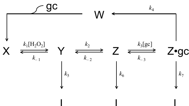
Figure A. Model of the inactivation of u-cytc550 by \text{H}_2\text{O}_2 . It is assumed that the inactivation step involves the conversion of peroxide-reacted intermediate, Y, Z or \text{Z} \cdot \text{gc} . No assumption is made which of these intermediates is the labile species (see text). Species W is the one-electron reduced reaction product of species Z. It is assumed not to be converted into inactivated protein, I.
