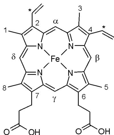
Figure 1.1. Heme b . The relevant carbons are numbered according to the Fischer nomenclature. The meso-carbons are indicated by \alpha - \delta . The asterisks on the vinyls indicate where in c -type hemes the porphyrin is covalently attached to two cysteine residues via thioether linkages.
