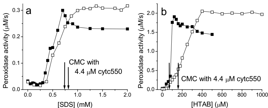
Figure 5.8. Protein concentration dependence of the detergent-induced peroxidase activity of cytc550. a) Peroxidase activity of 0.61 μM cytc550 (■) and 4.4 μM cytc550 (□) as a function of total added SDS. b) Peroxidase activity 0.61 μM cytc550 (■) and 4.4 μM cytc550 (□) as a function of total added HTAB. Each experiment was performed in 100 mM Na-phosphate pH 8, using 10 mM gc and 0.75 to 3 mM H 2 O 2 . Arrows indicate the CMC of SDS and HTAB, respectively. For both detergents, the CMC was higher in the presence of 4.4 μM cytc550.
