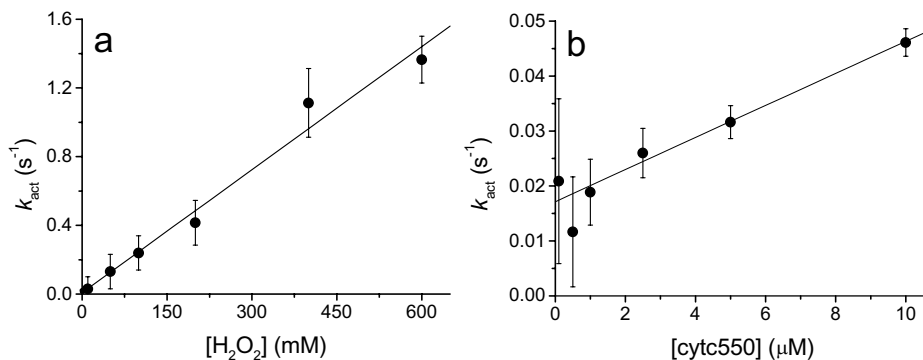
Figure 2.2. Rate of the peroxidase activity increase of cytc550 as a function of \text{H}_2\text{O}_2 (a) and cytc550 (b). The value of the activation rate constant, k_{\text{act}} , was obtained by fitting the first derivative of the product formation curve to a single exponential. Conditions: 25 mM gc and 1 μM cytc550 (a) and 5 mM \text{H}_2\text{O}_2 (b).
