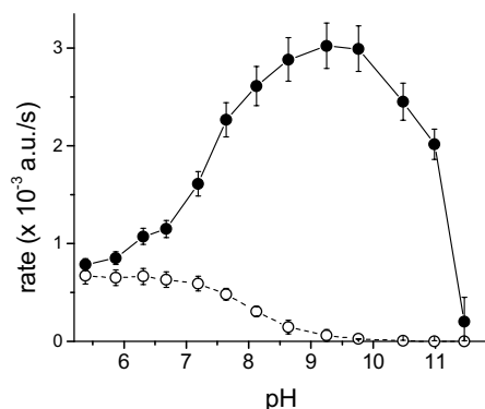
Figure 2.6. Dependence of the steady-state peroxidase reaction rate as a function of pH for cytc550 (●) and horse heart cytc (○). Conditions: 1 \mu M cytc, 10 mM \text{H}_2\text{O}_2 and 25 mM gc.
