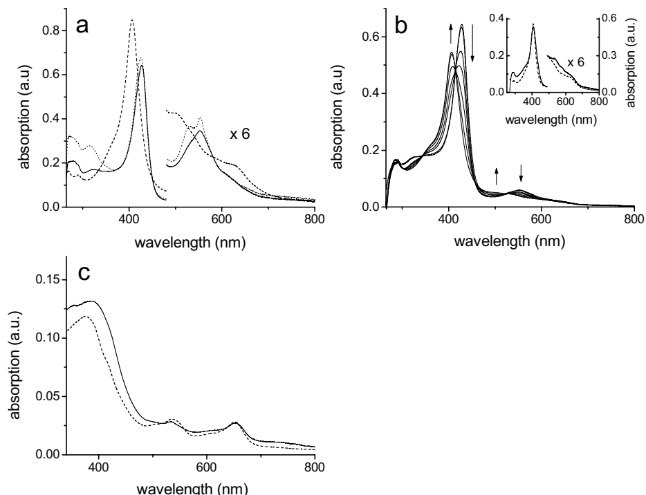
Figure 6.7. a) The UV-visible spectrum of u-cytc550 after addition of 3 equivalents H_2O_2 (dashed line), and after subsequent addition of sodium dithionite (solid line), and after addition of ethylmethylsulfide in the presence of sodium dithionite (dotted line). b) Spectral evolution of the sample obtained after addition of 3 equivalents H_2O_2 and subsequently exposed to several cycles of addition of sodium dithionite followed by O_2 . The arrows indicate the direction of the spectral changes following this treatment. Inset: the sample untreated and treated with a single cycle of dithionite/ O_2 , respectively. The left and right vertical scales are for untreated and treated sample, respectively. c) Spectrum (dashed line) of verdoheme-cytc550 in 6 M Gdn.HCl. This was prepared by a procedure similar to that described, [289] i.e. by prolonged exposure of u-cytc550 to 20 mM sodium ascorbate and a stream of O_2 . The solid line is the spectrum of the sample obtained after addition of 3 equivalents H_2O_2 and > 10 cycles of successive exposure to sodium dithionite and O_2 .
