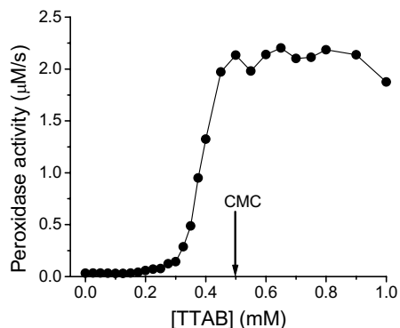
Figure 5.7. Peroxidase activity of cytc550 as a function of total added TTAB in 100 mM sodium phosphate pH 8. [Cyt550] was 0.61 \mu M, [gc] was 10 mM, [H_2O_2] between 0.6 and 30 mM. The arrow indicates the CMC determined for TTAB.
