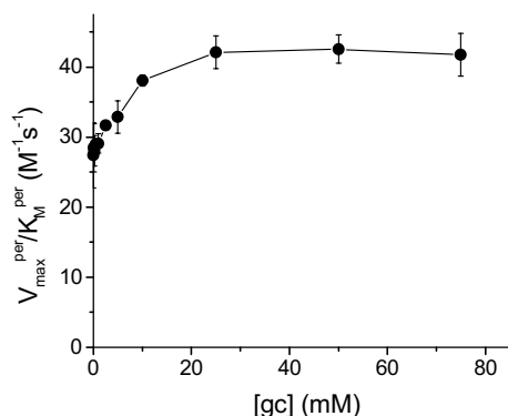
Figure 2.5. Inverse slope ( V_{\max}^{\text{per}}/K_M^{\text{per}} ) of plots of 1/\text{rate} vs. 1/[\text{H}_2\text{O}_2] as a function of [\text{gc}] . [\text{Cyt}550] was 1 \mu\text{M} .
