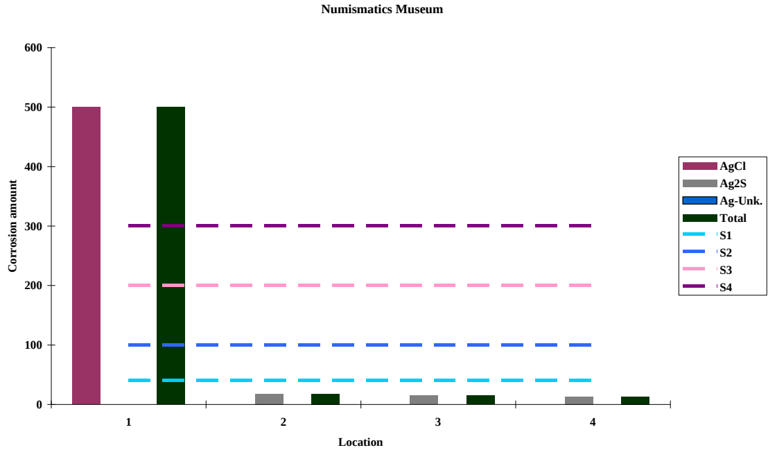
Figure 5.28 The ERC corrosion results of the silver film at the Numismatics Museum. The x-axis shows the location number where the measurement took place while the amount of corrosion is presented on the y-axis. The horizontal intermittent lines
