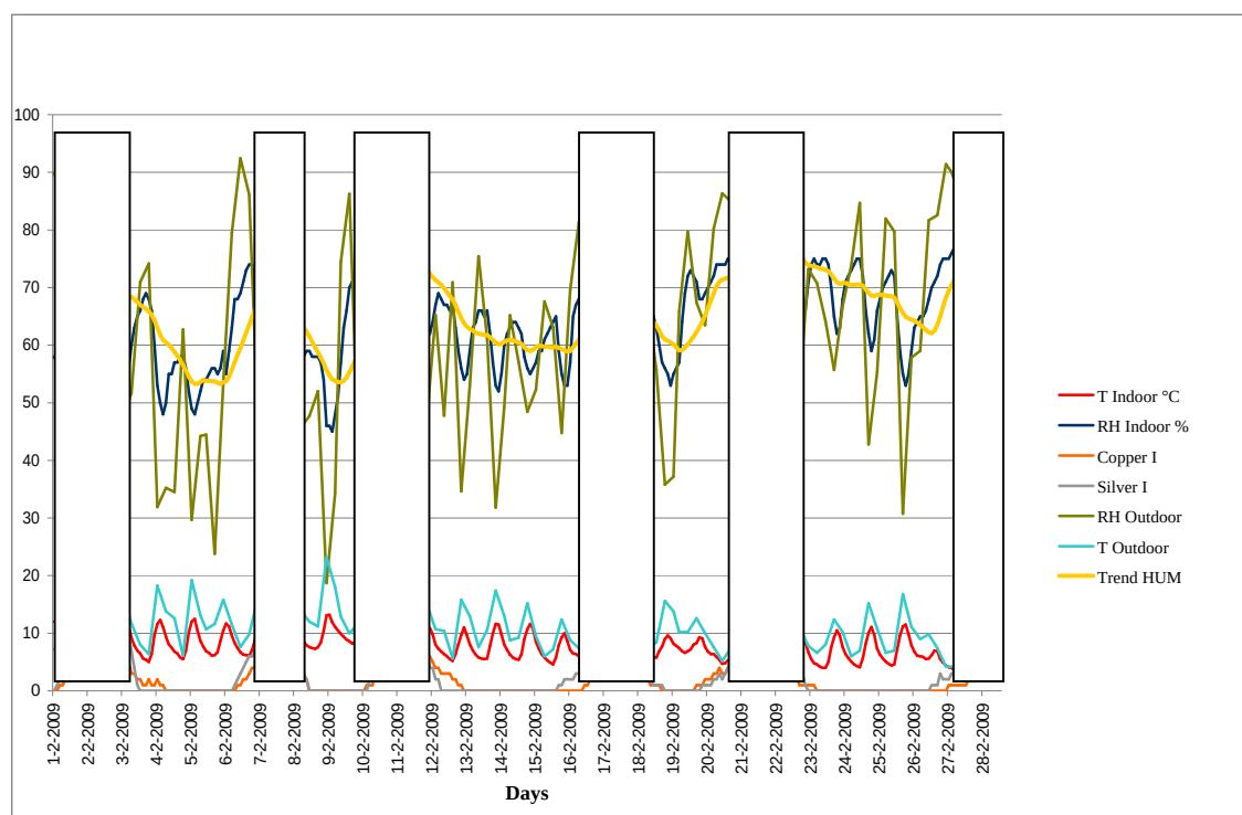
Figure 6.30 The relation between the indoor and outdoor environment compared to corrosion level at the DoAS, (winter monitoring).
