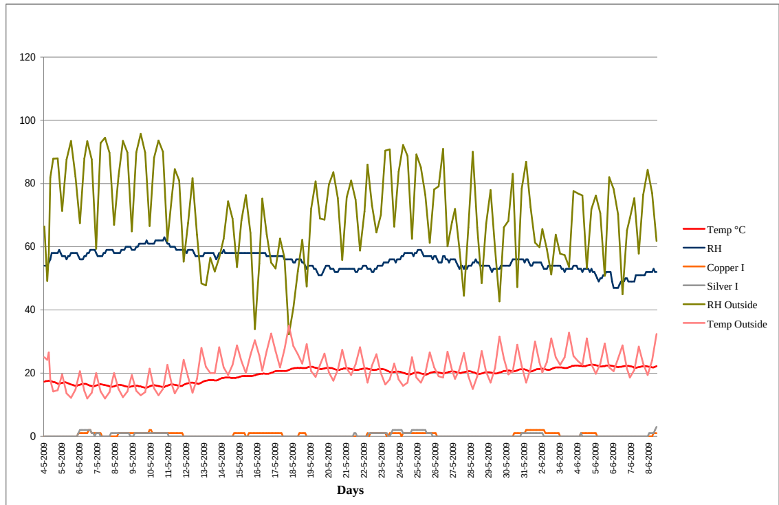
Figure 6.25 The correlation between fluctuations of the indoor and outdoor climates, in the Jordanian Heritage Museum and its' relation with the corrosion levels. The monitoring period was during the summer.
