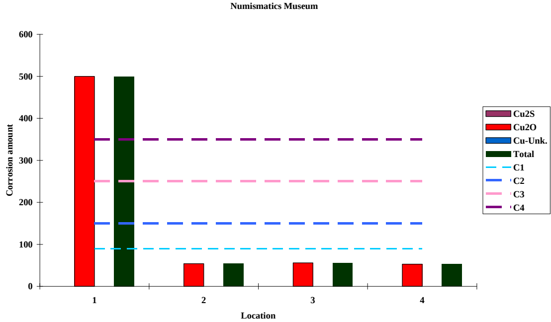
Figure 5.27 The ERC corrosion results of the copper film at the Numismatics Museum. The x-axis shows the location number where the measurement took place while the amount of corrosion is presented on the y-axis. The horizontal intermittent lines describe the levels of corrosion classifications, while the continual vertical lines indicate the concentration rate of the resulted copper corrosion in ? / 30 days.
