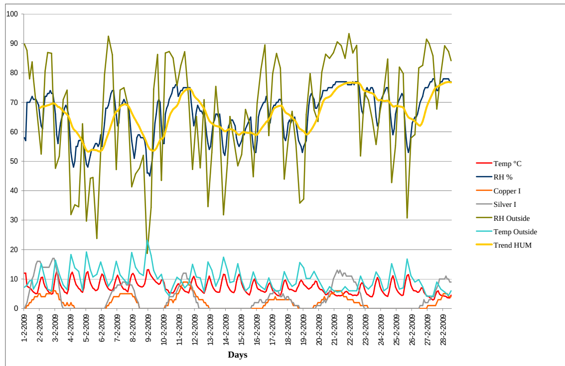
Figure 6.16 The correlation between the fluctuations of the indoor and the outdoor climates in the DoAS main storage in Amman and the relation to corrosion levels. The monitoring period was during the winter.
