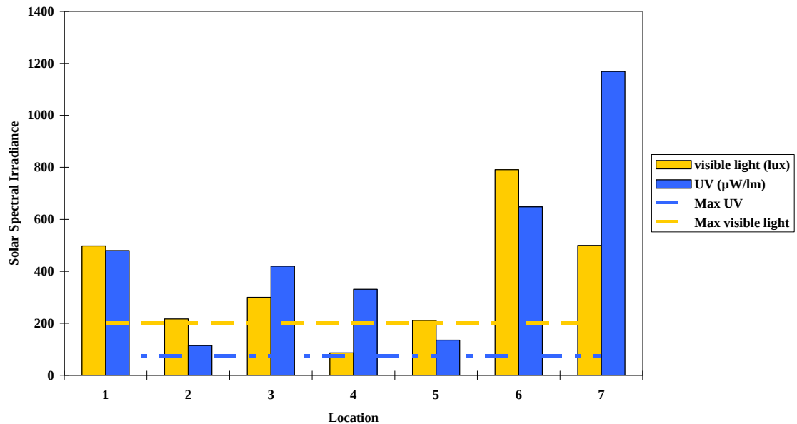
Figure 4.18 The average of the solar spectral irradiance readings at the Archaeology Museum within specific locations mentioned in Table 4.8.
