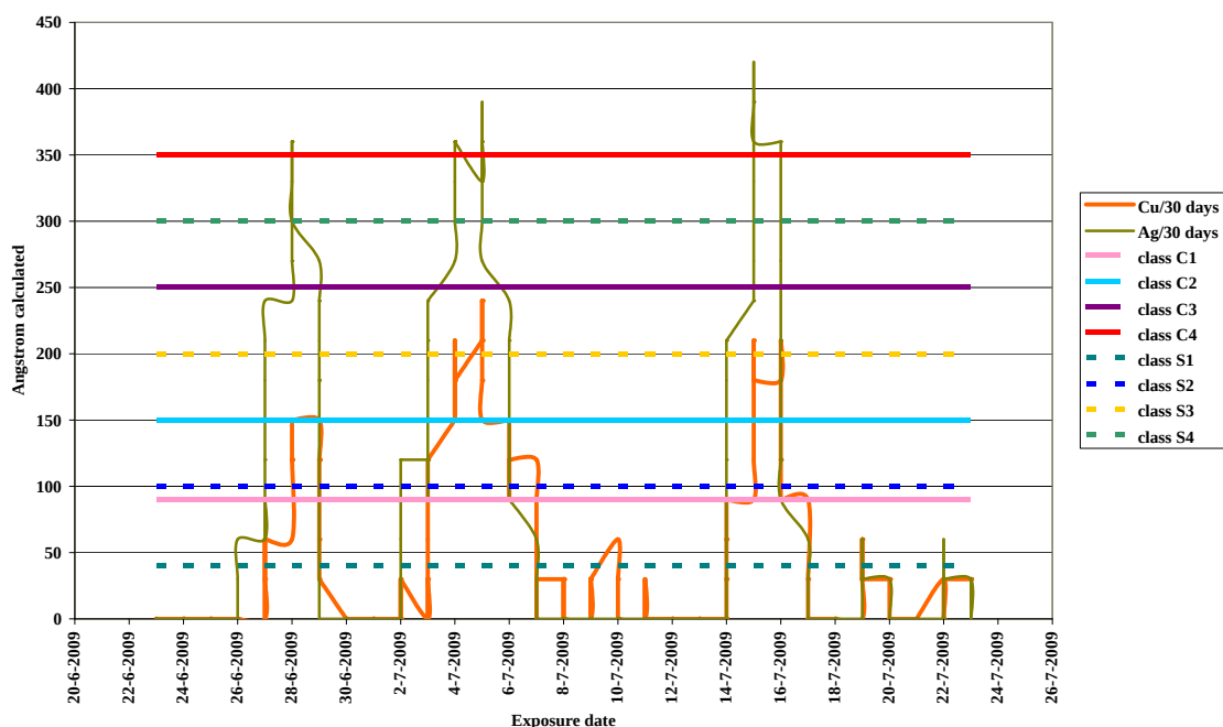
Figure 6.27 DoAS corrosion level compared to Muller's guidelines described in Table 6.4, (summer monitoring).
