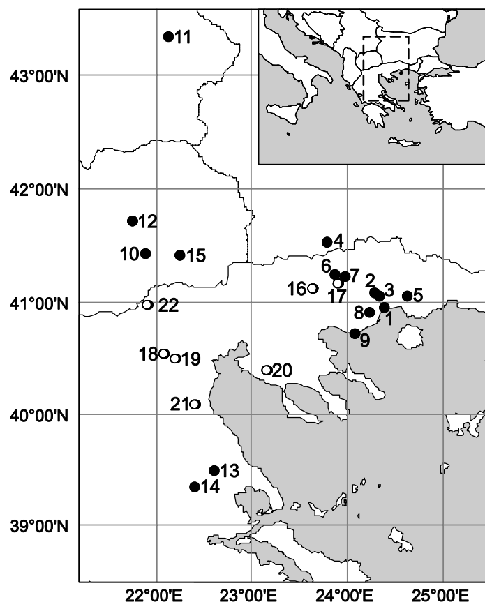
Figure 5.3. Distribution of sampling sites. Black dots refer to the localities of the ingroup samples; open circles to those of outgroup samples.
