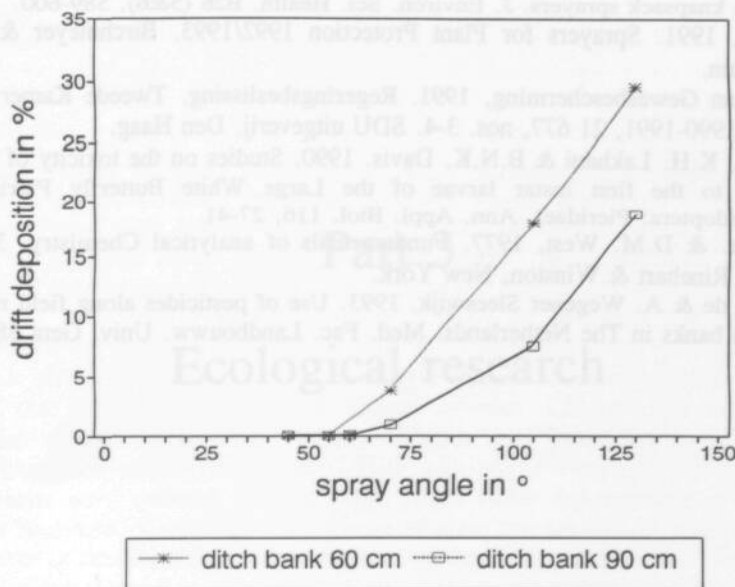
Figure 6. Relation between spray angle and drift deposition 0.6 m and 0.9 m down ditch bank at 5 m/s wind speed
