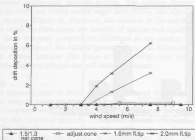
Figure 6. Drift deposition in ditches from different types of knapsack sprayers in relation to wind speed
