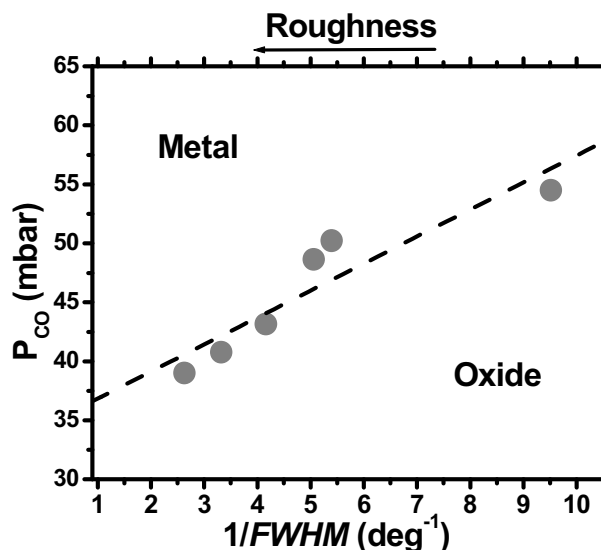
Figure 7: CO pressure at which the surface switches from the metallic phase to the oxide phase as a function of (FWHM)^{-1} of a rocking scan around the surface normal of the Pd(001) surface at (h\ k\ l) = (0\ 1\ 0.2) . This value scales approximately with the roughness, where a high roughness corresponds to a high FWHM, and hence a low value of (FWHM)^{-1} . Data are taken from the experiment shown in Figure 6 ( T = 460\ K , P_{O_2} = 480\ mbar ).
