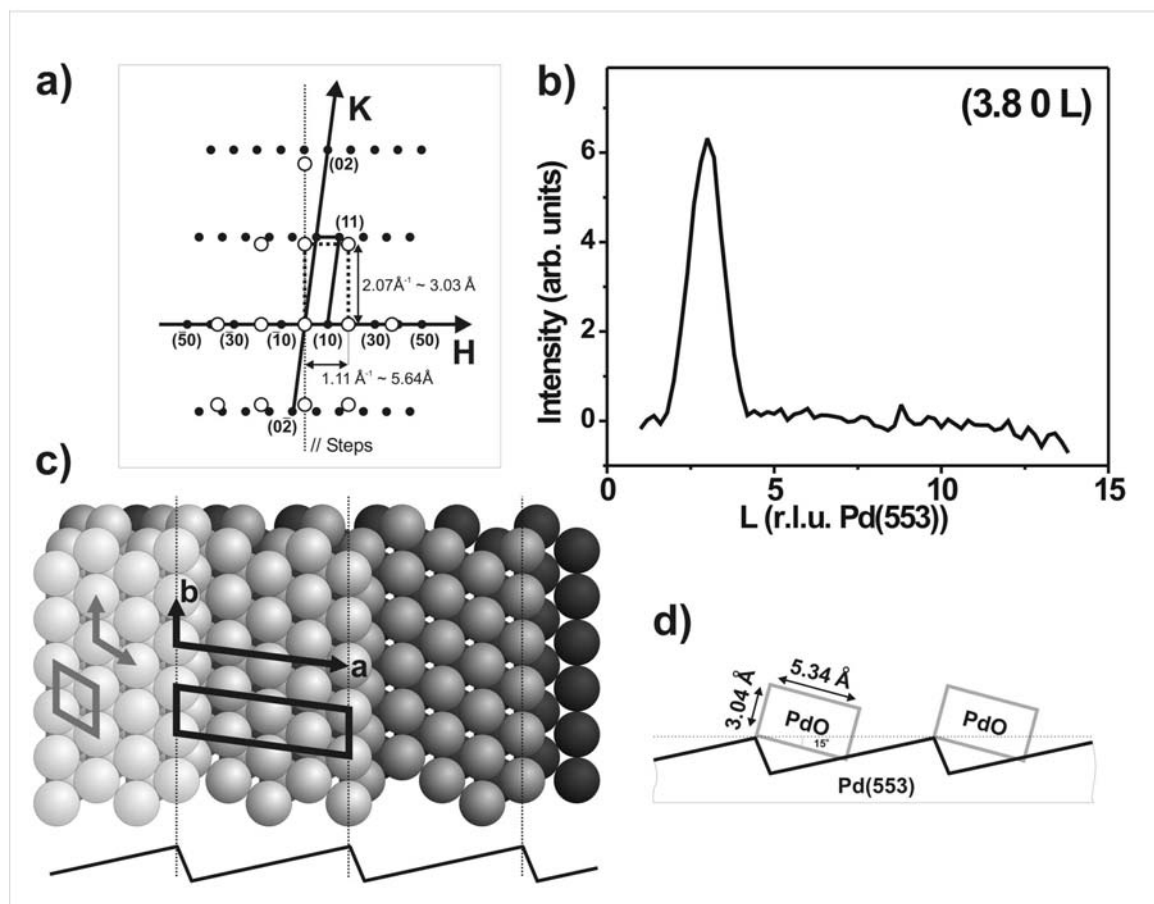
Figure 8: a): In-plane reciprocal space map of the Pd(553) (black dots) and the bulk-like PdO layer (hollow circles). All coordinates are given in reciprocal unit vectors of Pd(553) as described in this chapter. The PdO layer is incommensurate, but aligned along \mathbf{H} (the direction perpendicular to the step lattice), and along the steps. Due to the choice of the unit cell, the direction parallel to the steps is not \mathbf{K} but is given by the vector (2\mathbf{K}-\mathbf{H}) , and is marked by the dotted line. b): The diffraction intensity distribution along a rod of the PdO layer as a function of L at \mathbf{H} = 3.8 and \mathbf{K} = 0 . c) A ball model of the Pd(553) surface, and a schematic side view showing the height variation in the direction perpendicular to the step lattice. d) The model for the growth of the incommensurate bulk-like PdO, giving the dimensions of the PdO unit cells and the tilt angle with respect to the Pd(553)
