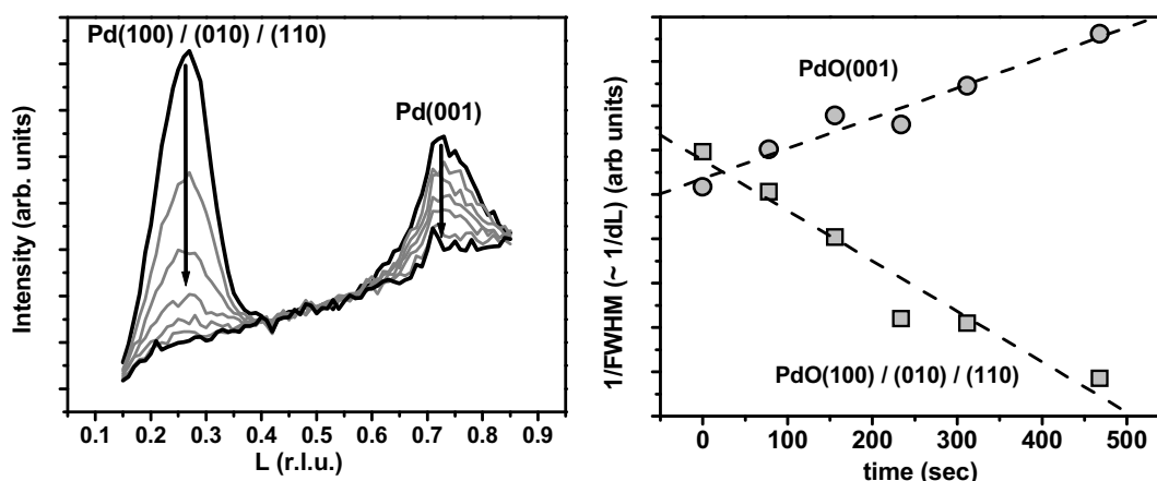
Figure 3: left panel: Intensity as a function of time of the (001) orientation (right) and (110) / (100) / (010) orientations (left) during exposure to a single pulse of CO ( P_{O_2} = 500 mbar, T = 475 K). Although both decrease in intensity, the diffraction peak of the (001) orientation grows smaller, but sharper, whereas the other peak widens and completely disappears. The width of the peaks is a measure for the ordered crystalline size of the different orientations. Right panel: Plotting this 1/\text{FWHM} as a function of time (and hence as a function of the total amount of CO oxidized on the surface) gives a clear view of the development of the different orientations during CO oxidation.
