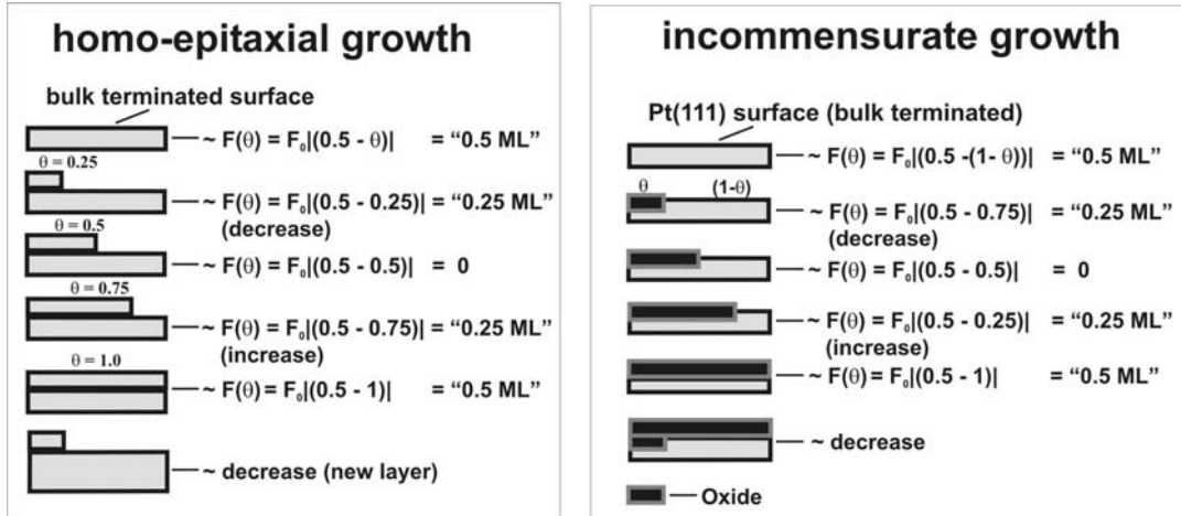
Figure 7: left panel: Schematic drawing of perfect, layer-by-layer homo-epitaxial growth (Frank – van der Merwe growth). Next to the model the behavior of F(\theta) as a function of the growth of that single layer is calculated. Right panel: Schematic drawing of the growth of an incommensurate layer on Pt(111). By taking atoms from the top layer of a bulk terminated crystal, and incorporating them in the incommensurate layer, material is ‘removed’ from this first layer. The coverage of the incommensurate \theta layer is the complement to the amount of material remaining in the top layer ( 1-\theta ). The behavior of F(\theta) as a function of the remaining material is calculated, and is exactly equal to the behavior of F(\theta) during homo-epitaxial growth.
