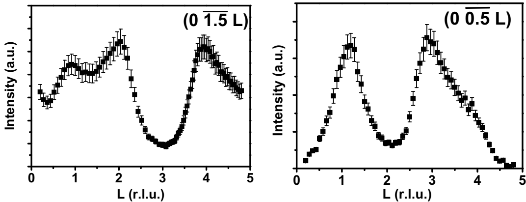
Figure 14: Distribution of diffracted intensity along the L direction for two non-equivalent superstructure rods of the 2x2 layer. The strong oscillation in intensity as a function of L indicates that more than one layer of Pt is involved in this 2x2 structure. Despite the gathered dataset, the structure of this layer has not been elucidated.
