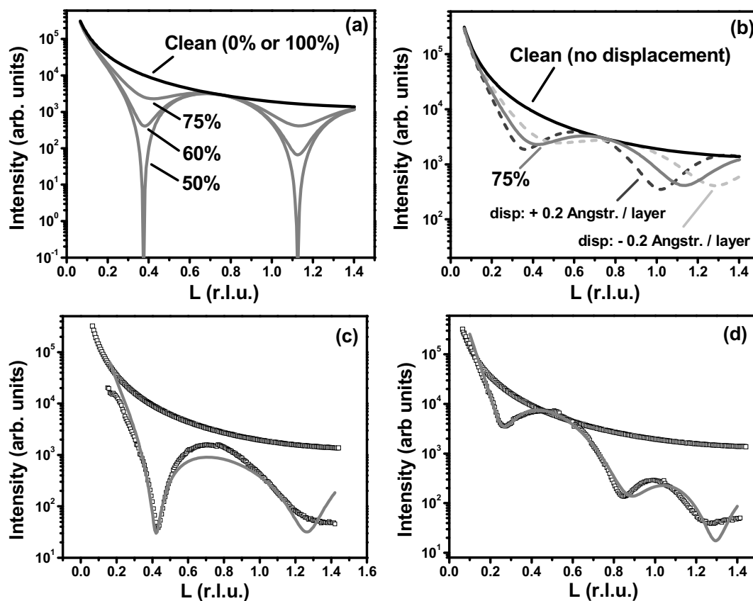
Figure 5: Simulations and real measured specular reflection data. a) A simulation of 4 layers of ‘oxide’ on a Pt(111) bulk terminated crystal. By varying the electronic density from 100% to 0% of the bulk electronic density the ‘depth’ of the oscillations along the 00L curve vary. b) Changing the position of the 4 oxide layers by stretching or contracting the interlayer distance within the oxide slab varies the period of the oscillations along the 00L curve (example given for a simulated oxide layer with an electronic density of 75% of bulk Pt(111)). c) Diffracted intensity for a relatively thin oxide layer on Pt(111), grown at 500 mbar of \text{O}_2 and 400 K, together with the diffracted intensity of a clean, smooth, bulk terminated Pt(111) surface. The grey line is the best fit, representing 1.5 ML of \alpha\text{-PtO}_2 . d) Diffracted intensity for a relatively thick oxide layer on Pt(111), grown at 500 mbar of \text{O}_2 and 580 K, together with the diffracted intensity from a clean, bulk terminated Pt(111) surface. The grey line is the best fit, representing 2.7 ML of \alpha\text{-PtO}_2 .
