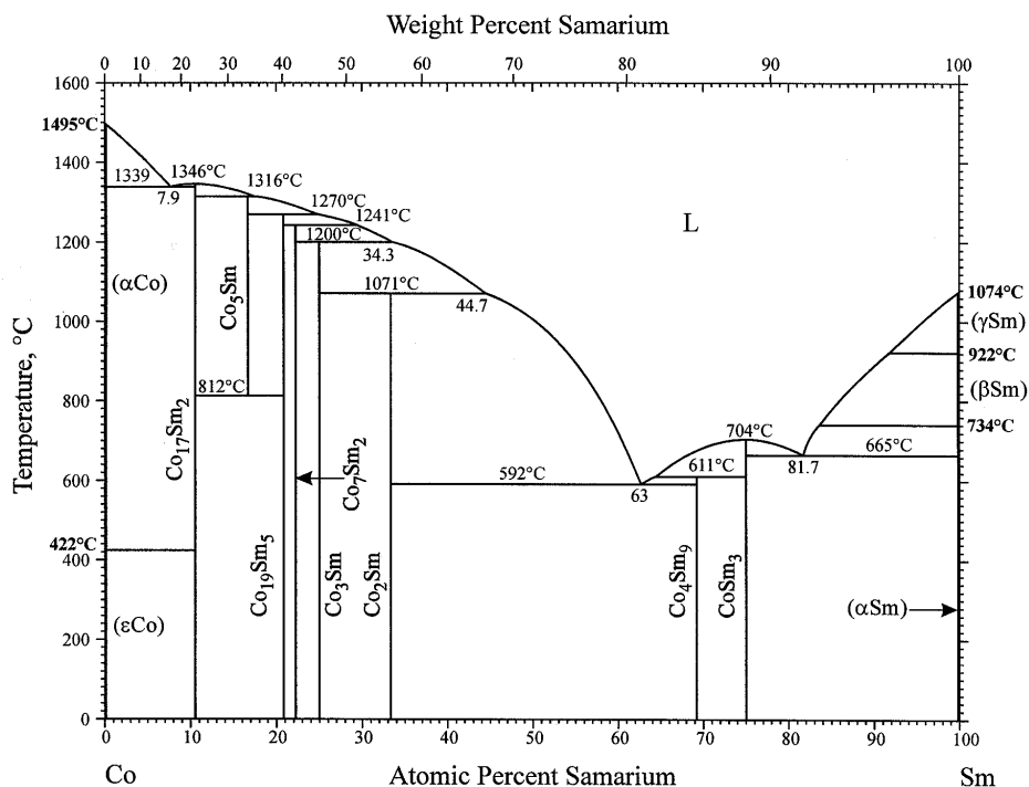
Figure 4.1: Sm-Co binary phase diagram [106]. Reprinted with kind permission from Springer Science and Business Media.
