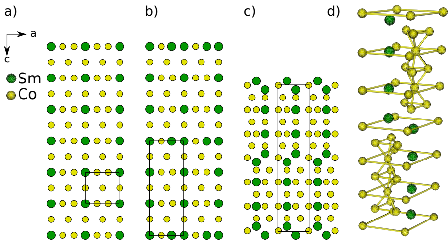
Figure 4.3: Construction of \text{Sm}_2\text{Co}_7 from \text{SmCo}_5 . In a), the \text{SmCo}_5 structure is shown, projected along the b -axis. In every third unit cell, a Sm atom is substituted for a Co-atom, as shown in b), whereafter a block of two \text{SmCo}_5 unit cells sandwiched between \text{SmCo}_2 unit cells is shifted by (\frac{2}{3}, \frac{1}{3}, 0) , as can be seen in c). In d), the \text{Sm}_2\text{Co}_7 unit cell is shown. Image d) made with the program Molekel [107].
