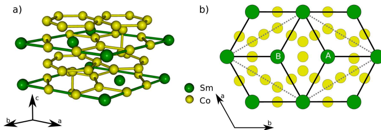
Figure 4.4: a) Structure of \text{Sm}_2\text{Co}_{17} , where in b) the atomic arrangement of a Sm sublattice in the basal plane is shown. The black lines indicate the \text{SmCo}_5 unit cell, where the gray dotted line indicates the \text{Sm}_2\text{Co}_{17} unit cell. Depending on the layer, a pair of Co atoms is at A and a Sm atom at B or vice versa. Image b) made with [107].
