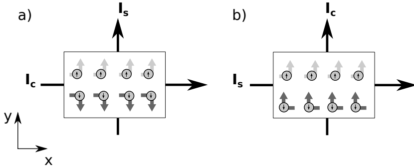
Figure 2.5: a) A spin current is induced by the spin Hall effect in a paramagnetic material. When sending a charge current in the x-direction, a spin current is generated in the y-direction due to the spin-orbit interaction. b) The inverse spin Hall effect induces a charge current in the y-direction when a spin current flows in the x-direction.
