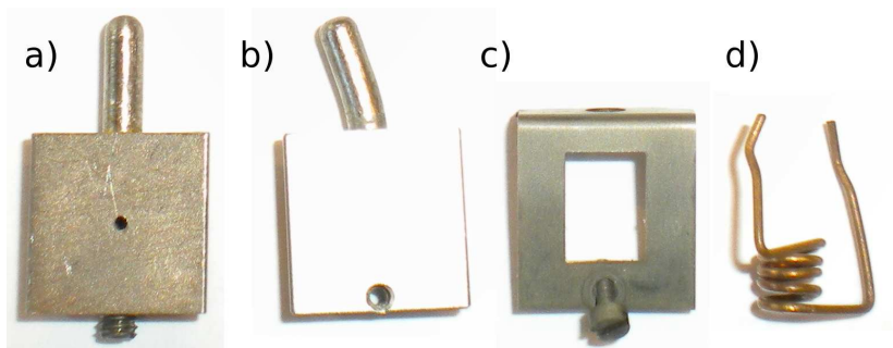
Figure 3.3: a) 9 \times 9 \text{ mm}^2 tip holder with on the bottom side the screw for tightening the mount of the tip wire. b) 9 \times 9 \text{ mm}^2 sampleholder onto which the substrate with the thin film or foil is glued. The hole in front of the sample holder is used to mount the Ti cap (c). For insulating substrates, a Ti cap (c) or Cu spring (d) are used to for making an electrical contact with the sampleholder.
