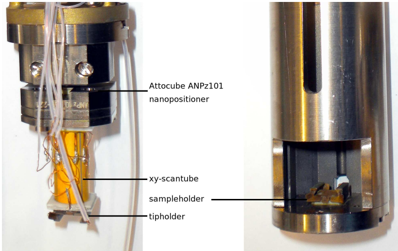
Figure 3.5: Point contact spectroscopy head based on the Attocube ANPz101 nanopositioner and a scan tube to scan in the x- and y-direction. The tipholder is mounted below the scan tube and the sample holder is mounted at the bottom of the protection cap, that is mounted around the piezo nanopositioners.
