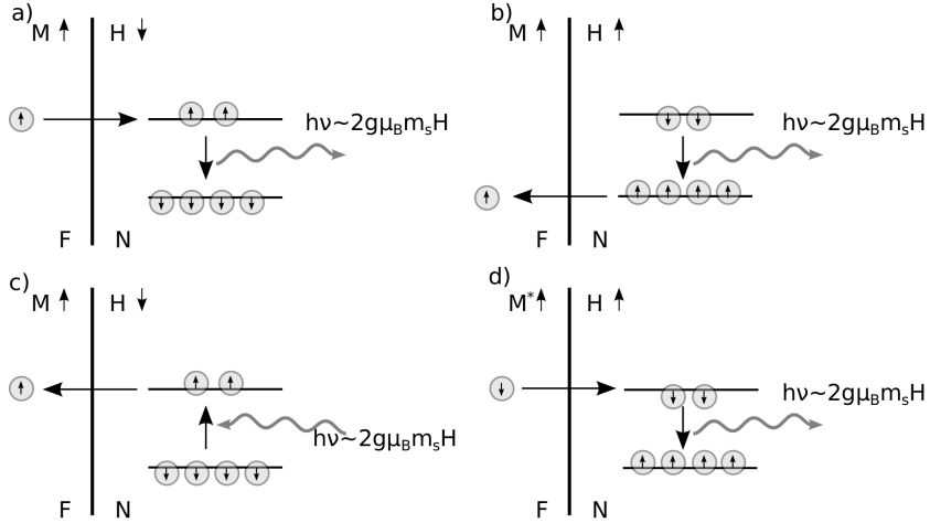
Figure 2.7: Four possible ferromagnet (F)/Normal metal (N) configurations, where a spin-flip process could generate a photon. In a), the magnetization M of F is antiparallel with the applied field H . Majority electrons are injected from F into N, leading to an inverse population of the Zeeman levels in N. A spontaneous or stimulated spin-flip process will emit a photon with the frequency proportional to the applied field H . b) When the magnetization M in F is parallel to the applied field H , electrons from the N layer are injected mostly in the majority band of F, resulting in an inversely populated Zeeman level in N. Again, a spontaneous or stimulated spin-flip process will emit a photon with the frequency proportional to the applied field H . In c), the magnetization M of F is antiparallel with the applied field H , but now the F/N bilayer is irradiated with photons with the energy equal to the Zeeman splitting. A spin-flip transition can be induced when a spin-down electron absorbs a photon. This will induce a photocurrent through the N into the F-layer. In d), the F layer is a minority type ferromagnet. When the magnetization M^* is parallel to the applied field, minority carriers will flow from the F into the N layer, creating an inversely populated Zeeman level. Again, a spontaneous or stimulated spin-flip process will emit a photon with the frequency proportional to the applied field H . Adopted from [74].
