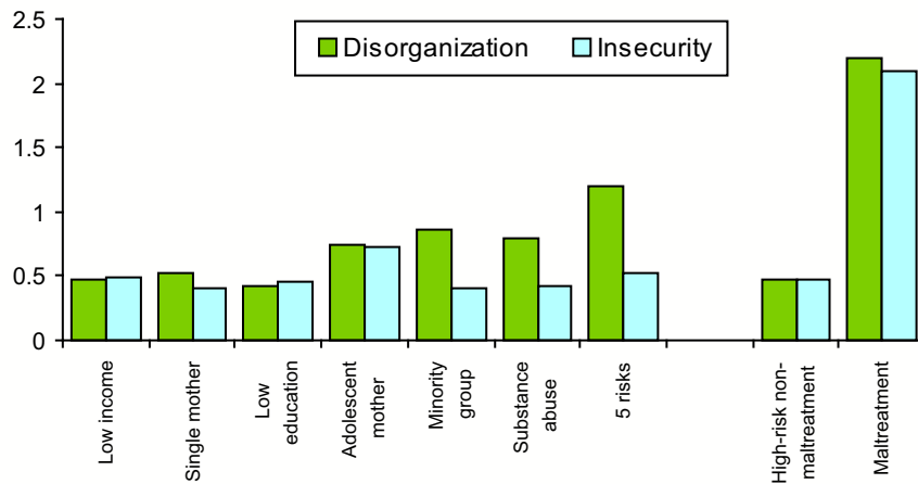
Figure 1. Combined Effect Sizes for Risk Indicators and Maltreatment Status
