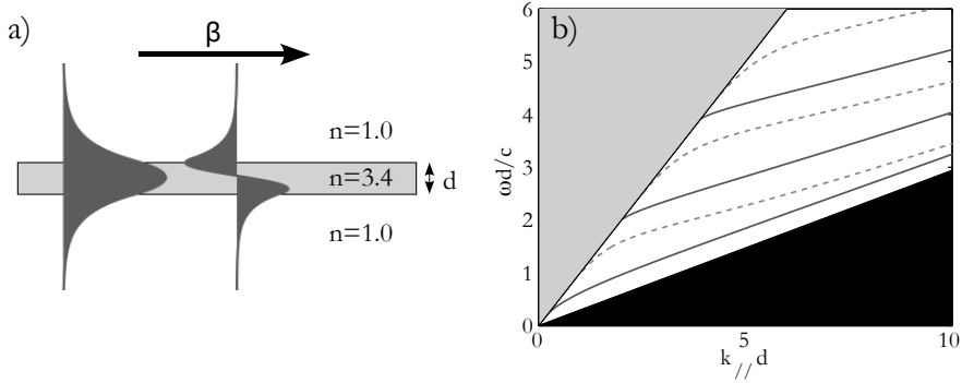
Figure 1.2. (a) Electric field distribution of the first two TE waveguide modes of a slab with refractive index n = 3.4 , surrounded by air. (b) Dispersion diagram of this structure. The solid and dashed curves give the dispersion of the TE and TM waveguide modes, respectively. The grey area indicates the light cone, where propagating solutions exist that are not bound to the slab. The black area indicates the region where no propagating modes exist at all.
