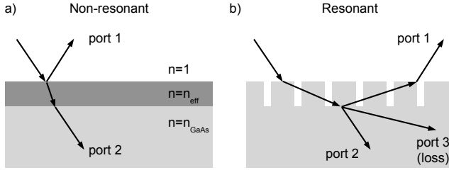
Figure 3.2. Model for the non-resonant (a) and resonant (b) channels in the model. The numbers indicate the different ports in the scattering matrix model. (a) The non-resonant channel is modeled by applying effective medium theory to the photonic-crystal layer and calculating the Fresnel reflection and transmission coefficients of the layered system. (b) For the resonant channel, the incident light is diffracted into a waveguide mode, which can diffract back to ports 1 and 2, but can also propagate into the substrate (port 3) constituting loss.
