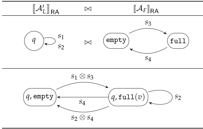
Figure 3.9: Composition of \llbracket \mathcal{A}'_L \rrbracket_{RA} and \llbracket \mathcal{A}_F \rrbracket_{RA} .
