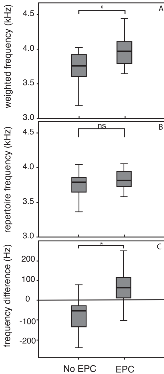
Figure 4.4. Males singing low frequency songs suffer less paternity loss. (A) Non-cuckolded males sing on average lower than cuckolded males during the dawn chorus at the peak of female fertility (LMM; F_{1,21} = 6.84 ; *P = 0.018 ). (B) Differences cannot be ascribed to non-cuckolded males having lower song types in their repertoire (LMM; F_{1,21} = 1.64 ; P = 0.22 ; peak frequencies of low notes averaged over song types of an individual's repertoire). (C) Differences are the result of using the lower song types more often (LMM; F_{1,21} = 7.39 ; *P = 0.014 ; difference between average weighted song frequency (A) and frequency averaged over repertoire (B) per individual).
