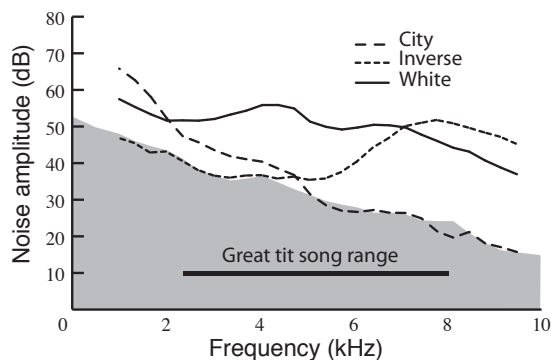
Figure 2.3. Energy distribution of noise stimuli. Power spectrograms illustrate the three noise treatments, averaged over experiments. Noise recordings made at the position of the focal bird were analysed in 26 adjacent frequency bands in the range of 1 – 10 kHz. The shaded area illustrates the spectrum of average background noise in our study area. Note that the normal background noise is added to the experimental noise which especially affects the ‘Inverse’ stimuli. Great tit song range is indicated by the black bar for comparison.
