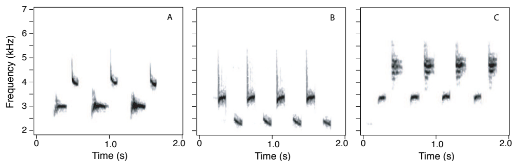
Figure 2.1. Three great tit song type examples from our study population showing variation in peak frequency of the low-notes and high-notes. The song types in these examples consist of two notes and are delivered in series called ‘strophes’. Song type frequency characteristics can vary discretely both within and between individuals. Song types B and C are recorded from the same individual and switching between these song types results in a low-note frequency change of 1.2 kHz.
