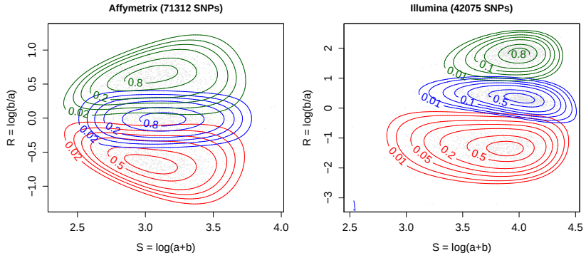
Figure 7.3: Raw data with estimated smooth densities. Left panel: a typical (symmetric) Affymetrix array. Right: a typical (asymmetric) Illumina array. Contours, normalized to 1, are overlayed for [0.02,0.05,0.1,0.2,0.5,0.8] (left) and [0.01,0.02,0.05,0.1,0.2,0.5,0.8] (right).
