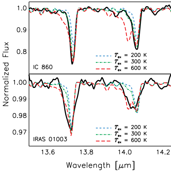
Figure 8.2 Illustration of the temperature sensitivity of the \text{C}_2\text{H}_2 and HCN Q -branch profiles in direct comparison to the observed spectra of IC 860 (best fit T_{\text{ex}} = 280 K) and IRAS 01003-2238 (best fit T_{\text{ex}} = 630 K). The shape of the Q -branch profile determines the derived excitation temperatures with an uncertainty of \sim 30\% . A better constrained error estimate is difficult to determine at the IRS resolution.
