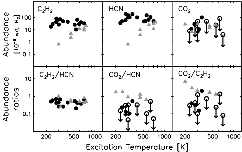
Figure 8.4 Top : Observed C 2 H 2 , HCN, and CO 2 abundances using a total H 2 column obtained from the 9.8 \mu m silicate absorption band. Bottom : Abundance ratios of C 2 H 2 , HCN and CO 2 . Both the absolute abundances and the abundance ratios are indicated with circles and are presented as functions of excitation temperature. Included are the observed values toward a sample of Galactic massive YSOs (Boonman et al., 2003; Lahuis & van Dishoeck, 2000) plotted with grey triangles. The derived absolute abundances toward the (U)LIRGs show significant enhancements in the abundances of C 2 H 2 and HCN for sources with excitation temperatures below 500 K. The C 2 H 2 /HCN abundance ratios are quite similar however, the CO 2 /C 2 H 2 and CO 2 /HCN ratios toward the (U)LIRGs are systematically lower than toward the Galactic massive YSOs, suggesting that a different chemistry may apply.
