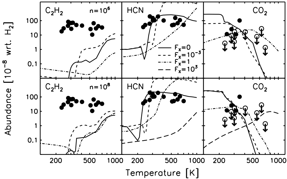
Figure 8.3 Results of equilibrium X-ray-enhanced chemical models for the three observed molecules. The calculated abundances are shown for moderate ( 10^6 \text{ cm}^{-3} ) and high density ( 10^8 \text{ cm}^{-3} ) and for four X-ray flux levels ( F_x = 0, 10^{-3}, 1 and 10^3 \text{ erg cm}^{-2} \text{ s}^{-1} plotted with solid, dashed, dot-dashed, and long-dashed lines, respectively). Note that except for HCN and \text{CO}_2 at high density, the abundances for the highest X-ray flux are below the plotted range. Overplotted are the observed abundances. Details of the model can be found in Stauber et al. (2005); Stauber et al. (2006).
