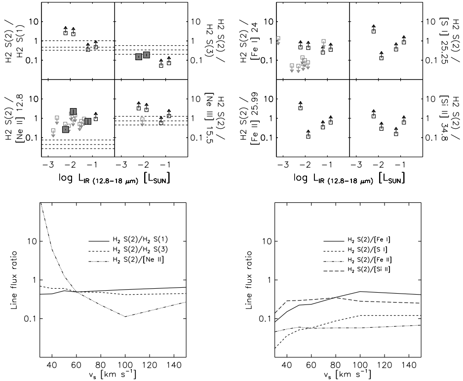
Figure 5.10 Line ratios of H 2 S(2) w.r.t. other species as functions of the mid-IR luminosity. Large filled symbols are used for sources with both H 2 S(2) and the second line detected. Small open symbols with arrows indicate lower and upper limits of the line ratios. The dashed lines in the left plot show the line ratios for the predictions from the Glassgold et al. (2007); Nomura et al. (2007) models. The lower two plots show the ratios from shock models by Hollenbach & McKee (1989) for different shock velocities.
