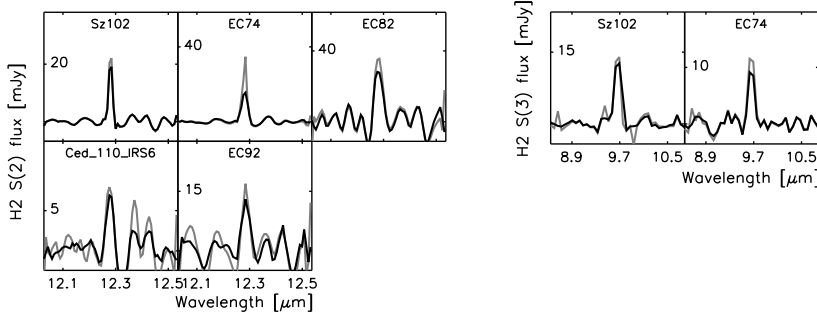
Figure 5.5 Detection of \text{H}_2 lines toward the c2d sample of T Tauri stars with disks. Only a few of the 76 sources show clear detections. Plotted in gray is the total observed emission (compact source + extended component) and in black the emission after correction of the estimated extended emission.
