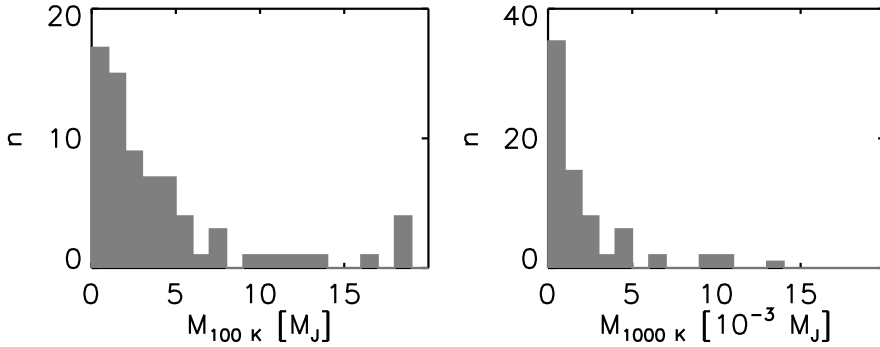
Figure 5.7 Distribution of \text{H}_2 mass upper limits derived for 100 and 1000 K gas. The bottom two panels are blow-ups with a smaller binsize of the upper panels.
