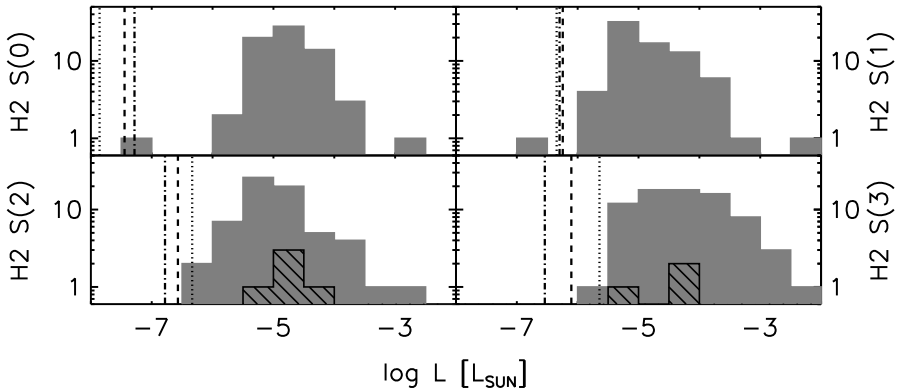
Figure 5.6 Observed line strengths (hatched bars) and upper limits (solid gray bars). The vertical lines present model T Tauri disk line strengths of \text{H}_2 S(0), S(1), S(2), and S(3) from Nomura et al. (2007). The models incorporate UV and X-ray heating of the circumstellar disk for three grain size distributions ( a_{\text{max}} = 10\mu\text{m} , 1mm, and 10cm represented by dotted, dashed, and dashed-dotted lines respectively). For S(0) the line strength increases with increasing maximum grain size, while for S(2) and S(3) the line strength decreases as the maximum grain size increases.
