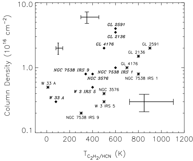
Figure 4.9 Column densities of \text{C}_2\text{H}_2 and HCN as functions of their excitation temperature. The column densities of \text{C}_2\text{H}_2 are shown as asterisks and the column densities of HCN as diamonds.
