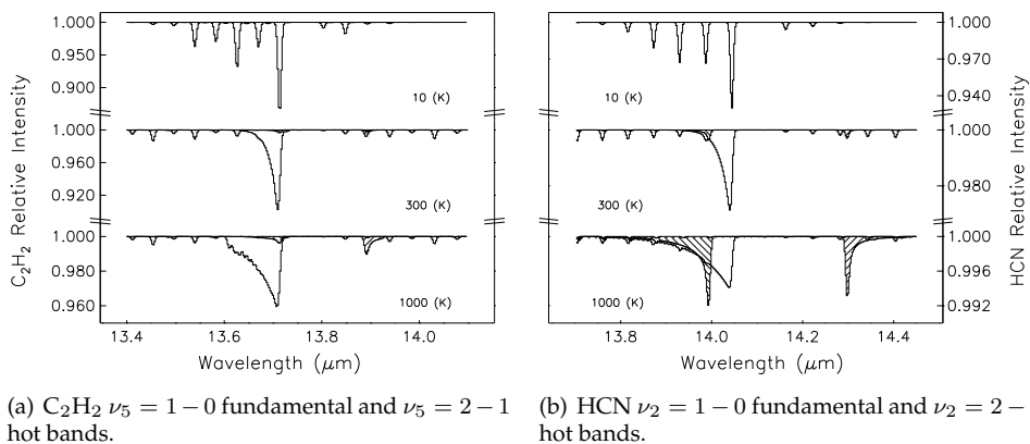
Figure 4.4 Examples of the fundamental 1 – 0 band and the 2 – 1 hot bands of the \nu_5 C 2 H 2 band (Figure 4.4(a)) and the \nu_2 HCN band (Figure 4.4(b)). For both molecules the synthetic spectra are shown for temperatures of 10, 300 and 1000 K at a column density of 1.10^{16} \text{ cm}^{-2} , R = 1800 and b=5 \text{ km s}^{-1} . The shaded regions indicate the hot band absorptions (see Tables 4.2 and 4.3 for details). Note the difference in scale between Figure 4.4(a) and 4.4(b). In particular, note the \nu_5 = 2 - 1 C 2 H 2 hot band at 13.89 \mu\text{m} . Although it is relatively weak compared to the fundamental \nu_5 = 1 - 0 C 2 H 2 band its strength is of the same order as the \nu_2 HCN bands.
