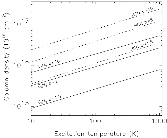
Figure 4.3 Column densities at which the strongest C_2H_2 and HCN absorption lines become optically thick ( \tau = 1 ) for Doppler parameters b of 1.5, 5 and 10 km s -1 at excitation temperatures from 10 to 1000 K.
