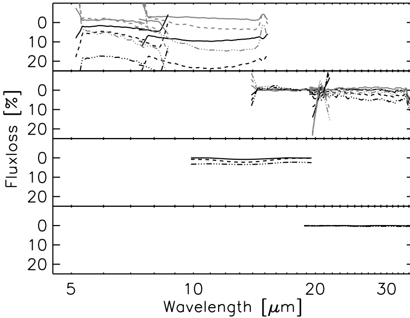
Figure 3.12 Pointing error flux loss for 0.4, 0.8, and 1.2''. The SL and LL fluxloss functions are derived from standard star mapping observations, the SH and LH fluxloss functions are derived from the optimal extraction cross dispersion PSF assuming a spherical PSF. Empirical fluxloss functions for SH and LH are to be derived at a later date. For SL and LL it should be noted that the PSF is not centered on the slit and two curves are plot for each offset, for a positive and a negative pointing error. The characterization of the pointing fluxloss is a collaborative effort of the c2d and FEPS legacy teams.
