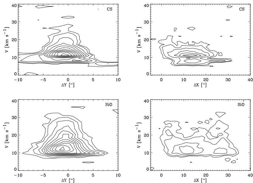
Figure 8.5. CS (upper) and SiO (lower) position-velocity maps for the IRAS2A shock. The coordinate frame has been rotated and translated to an XY-coordinate system with the X-axis along the propagation direction of the outflow ( \sim 19^\circ with the RA axis in Fig. 8.2) and the Y-axis in the perpendicular/north direction. The (0,0) point for the XY coordinate system has been chosen to be at ( 87'' , -23'' ) i.e., at the working surface, or head, of the outflow as judged from the morphology of the high velocity emission. The contours are given at 2\sigma , 4\sigma , 8\sigma , ... and upwards in steps of 4\sigma .
