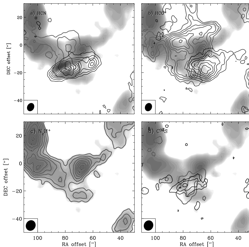
Figure 8.3. Moment maps for the lines observed at BIMA: a) HCN, b) HCO + , c) N 2 H + and d) C 34 S. As in Fig. 8.2 the black/grey dotted and black solid lines indicate low and high velocity material, respectively (the low velocity emission is integrated over 5–9 km s -1 and the high velocity emission over 9–16 km s -1 ). The contours ascend in steps of 3σ and are overlaid on grey-scale images of the low velocity N 2 H + emission.
