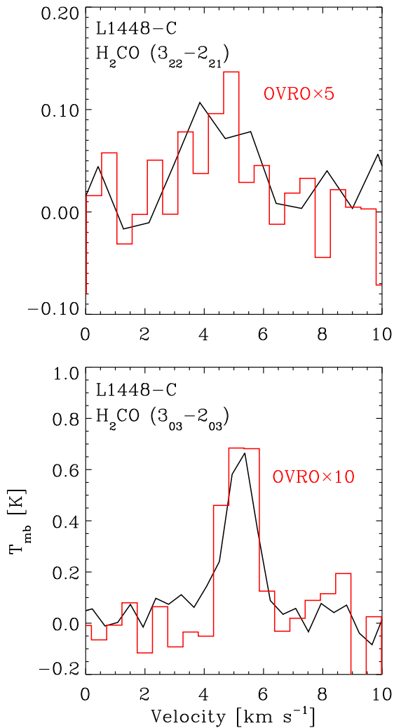
Figure 7.8. Comparison between the H 2 CO line emission towards L1448-C, at the source position, from JCMT single-dish observations (line diagram) and OVRO interferometric observations (histogram) restored with the JCMT beam (22"). The OVRO spectrum has been scaled in order to account for the flux seen in the JCMT spectrum.
