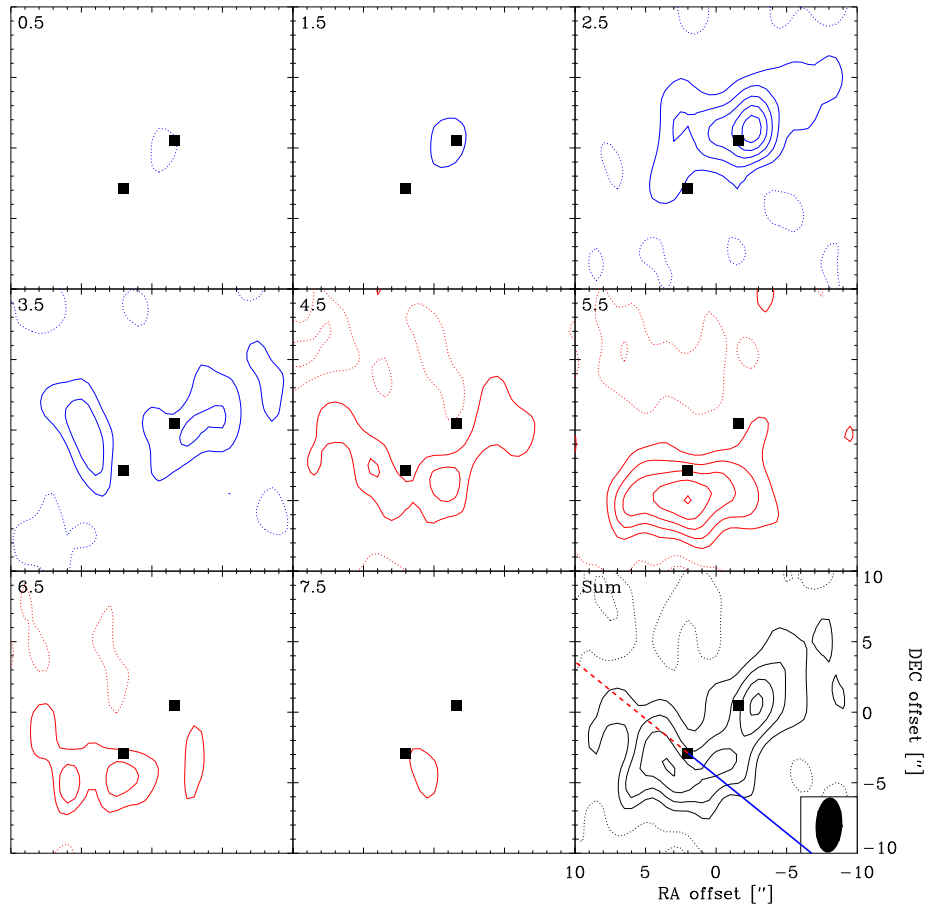
Figure 7.16. OVRO interferometer maps of H 2 CO 3 03 → 2 02 line emission (contours) for IRAS 16293–2422. The H 2 CO emission has been separated into bins of 1 km s -1 and contours are in steps of 0.4 Jy beam -1 km s -1 (2σ). In the panel with the velocity-integrated line intensity the contours start at 1.0 Jy beam -1 km s -1 (2σ). Also indicated are the positions of the two continuum sources as well as the red- (dashed) and blue-shifted (solid) parts of the outflow.
