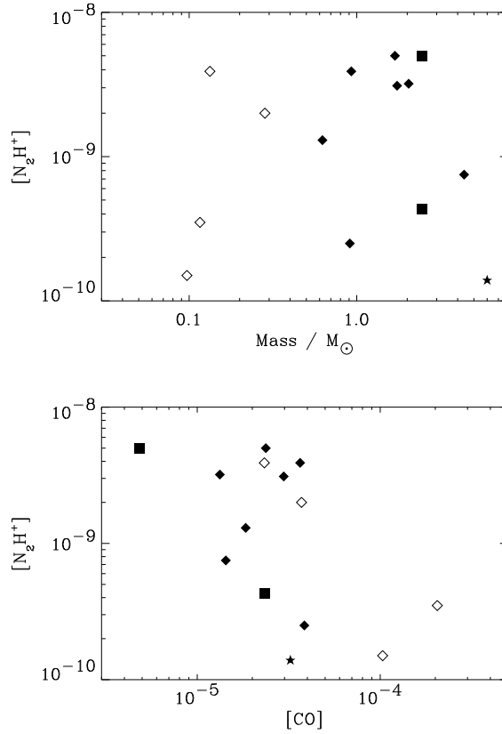
Figure 3.15. N_2H^+ abundance vs. mass (upper panel) and vs. CO abundance (lower panel). Symbols as in Fig. 3.12.
