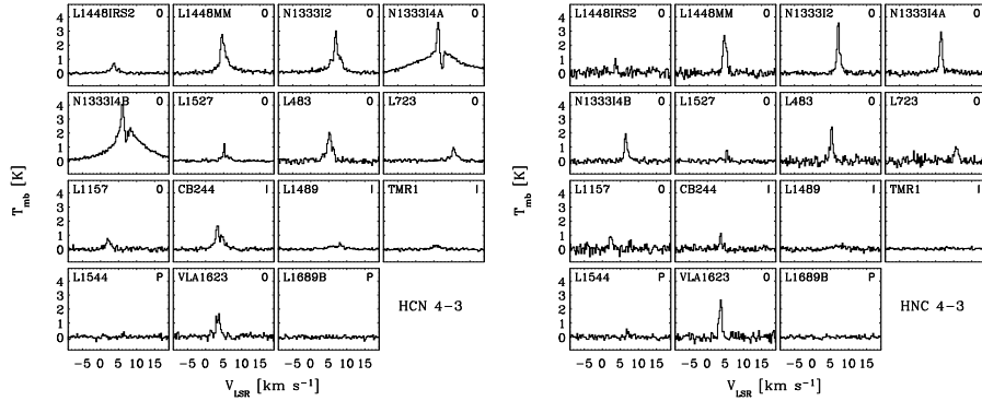
Figure 3.3. Spectra of HCN (left) and HNC (right) J = 4 - 3 from JCMT observations.
