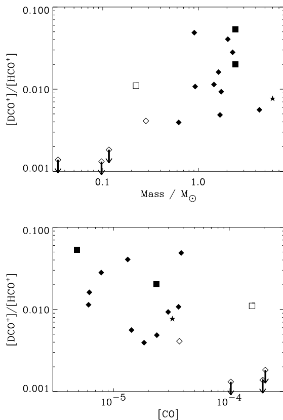
Figure 3.22. [DCO^+]/[HCO^+] ratio vs. mass (upper panel) vs. and [CO] (lower panel). Symbols as in Fig. 3.12.
