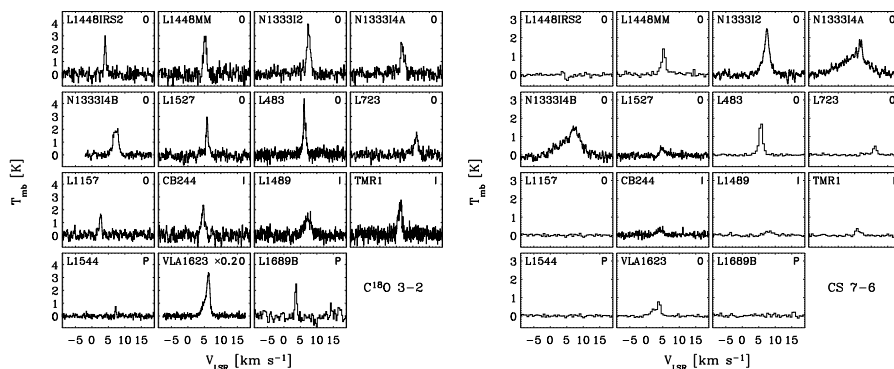
Figure 3.1. Spectra of C^{18}O J = 3 - 2 (left) and CS J = 7 - 6 (right) from JCMT observations. In this figure, and Fig. 3.2-3.4, the classes of the individual objects are indicated in the upper right corner of each plot by “0” for the class 0 objects (envelope mass > 0.5M_{\odot} ), “I” for the class I objects (envelope mass < 0.5M_{\odot} ) and “P” for the pre-stellar cores.
