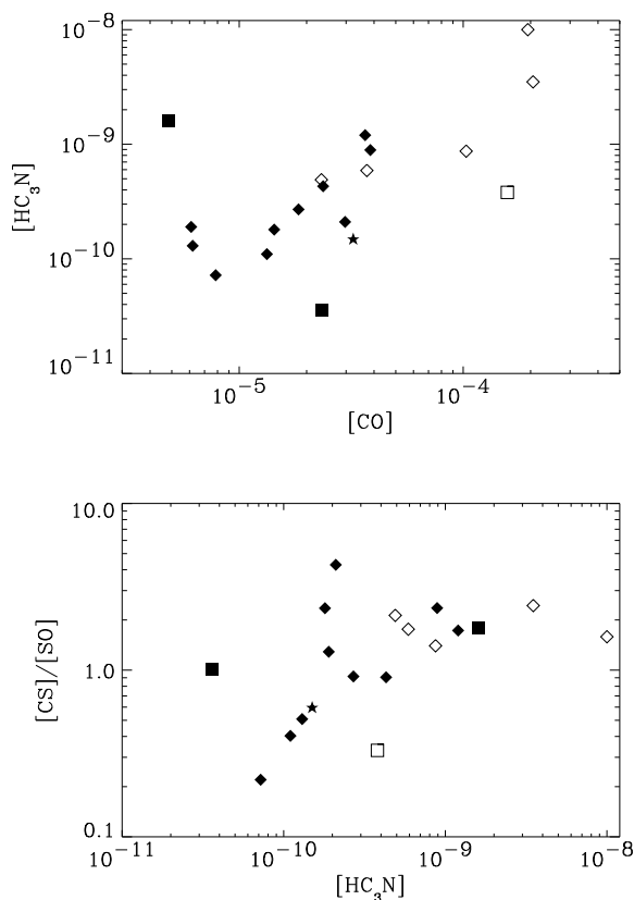
Figure 3.20. [HC_3N] vs. mass and [CO] (upper panel) and vs. [CS]/[SO] ratio (lower panel). Symbols as in Fig. 3.12.
