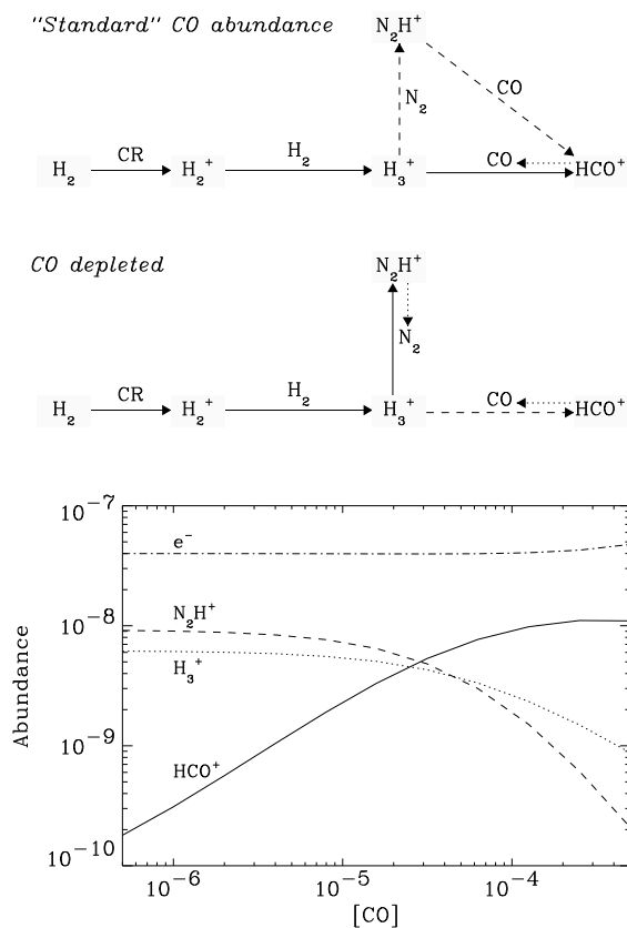
Figure 3.16. Upper panel: the chemical networks for low CO abundances (i.e., depletion) and standard CO abundance ( [\text{CO}] \sim 10^{-4} ). The dominant reactions are indicated by solid arrows, secondary reactions by dashed arrows. Where dissociative recombination is the main destruction for a molecule (i.e., \text{N}_2\text{H}^+ or \text{HCO}^+ ) this has been indicated by a dotted arrow. Lower panel: the electron, \text{N}_2\text{H}^+ , \text{H}_3^+ , and \text{HCO}^+ abundances as functions of CO abundance in a cell with density n(\text{H}_2) = 1 \times 10^6 \text{ cm}^{-3} and temperature T = 20 \text{ K} .
