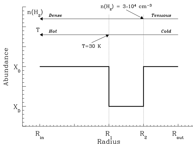
Figure 3.6. Simulated abundance profile in “drop” models.
