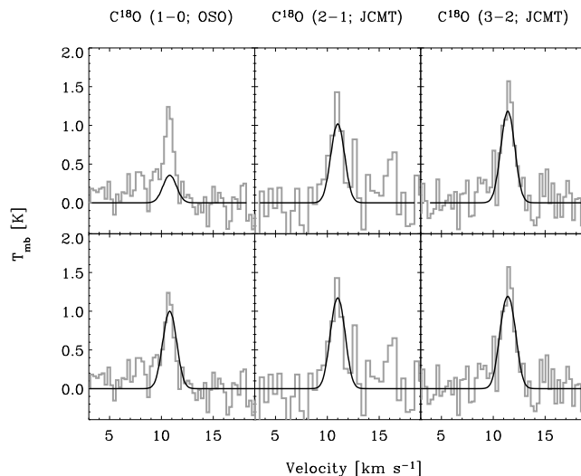
Figure 3.7. Fitted C^{18}O line-profiles for L723. Upper panels: constant fractional abundance of 3.9 \times 10^{-9} from Jørgensen et al. (2002). Lower panels: drop model with abundances of X_0 = 2.0 \times 10^{-7} for the undepleted material (with either temperatures higher than 30 K or densities lower than 3 \times 10^{-4} \text{ cm}^{-3} ) and an abundance of X_D = 1.5 \times 10^{-8} for material with CO frozen out.
