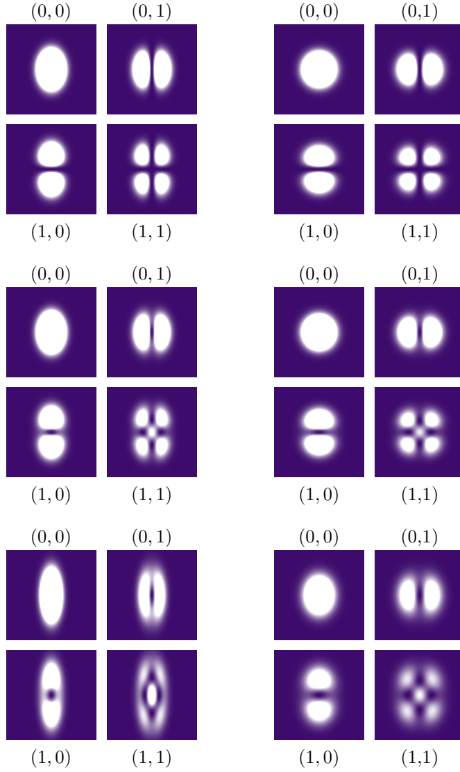
Figure 3.3: Intensity patterns of the (0,0) , (0,1) , (1,0) and (1,1) modes of the cavity between a stationary spherical and a rotating astigmatic mirror for different values of the rotation frequency \Omega . The plots in the left column show the intensity patterns near the spherical mirror while the plots in right column show the intensity pattern near the astigmatic mirror. The radius of curvature of the spherical mirror is 4L , where L is the mirror separation. The radius of curvature of the astigmatic mirror in the horizontal direction of the plot is equal to 2L while its radius of curvature in the vertical direction is 20L . From the top to the bottom the rotation frequency is increased from \Omega = 0 to \Omega = c\pi/(30L) and \Omega = c\pi/(6L) .
