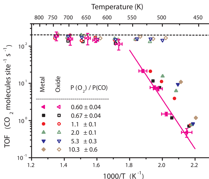
Figure 3.4: Arrhenius plot of the \text{CO}_2 production rate over Pd(100) at different P_{\text{O}_2}/P_{\text{CO}} ratios. The total gas pressure in the reactor was kept constant at 200 mbar, the partial CO pressure was kept constant at 10 \pm 1 mbar. Oxygen and Argon were mixed in the flow to obtain the desired P_{\text{O}_2}/P_{\text{CO}} ratio. Representative error bars and a fit of the Arrhenius behavior are shown for the P_{\text{O}_2}/P_{\text{CO}}=0.6 data set. The surface structure was determined simultaneously with the TOF by surface x-ray diffraction. Open symbols denote where the SXRD measurements showed the presence of an oxide (surface oxide, bulk-like oxide, or powder pattern) and solid symbols indicate under which conditions SXRD measured an oxide-free metal surface.
