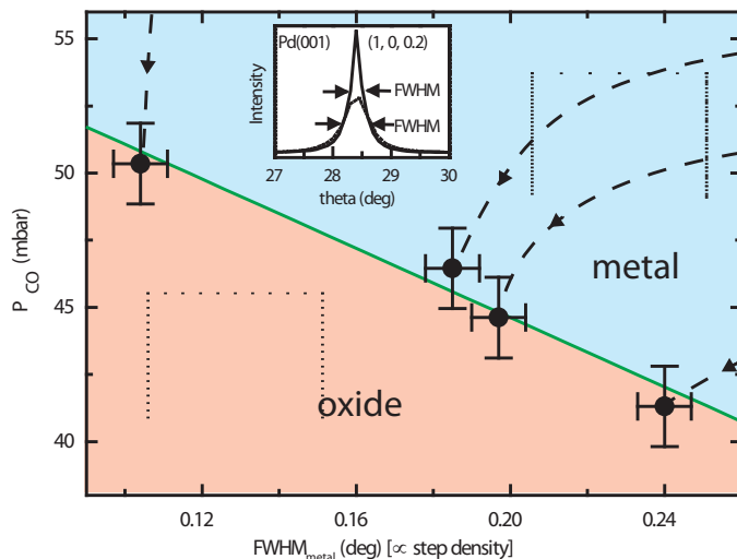
Figure 4.2: Stability diagram of the Pd(100) surface measured with surface x-ray diffraction. Measurements were performed at a temperature of 460 K in a CO/O 2 gas mixture with a fixed oxygen partial pressure of P_{O_2} = 0.48 bar in a batch reactor. The parameter along the horizontal axis of the main figure is the \text{FWHM}_{\text{metal}} of the diffraction peak on the metal surface with reciprocal coordinates (h, k, l) = (1, 0, 0.2) immediately prior to the metal-to-oxide transition. This peak width is a sensitive measure of the density of steps on the metal surface. The trajectories of (\text{FWHM}_{\text{metal}}, P_{\text{CO}}) approaching the metal-oxide transition are indicated by the four dashed curves. The error margins reflect the maximum variations observed in the peak width and the CO pressure at the transition. The inset shows two diffraction peaks on a trajectory at different \text{FWHM}_{\text{metal}} .
