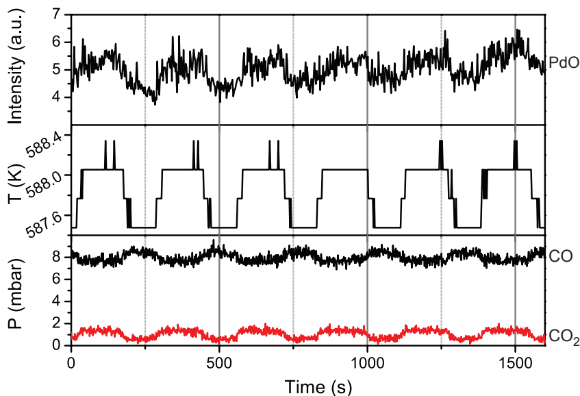
Figure 5.4: Spontaneous oscillations in the CO oxidation rate on the 15 nm diameter Pd particles supported on \text{SiO}_2 as measured by XRD and mass spectrometry. Measurements were performed in a constant flow of a \text{CO/O}_2/\text{Ar} gas mixture with an \text{O}_2 pressure of 210 mbar, an argon pressure of 281 mbar and a CO pressure of 9 mbar flowing at 50 \text{ ml}_n \text{ min}^{-1} . The mass spectrometry signals from CO and \text{CO}_2 show that the reaction rate oscillates (lower panel), which in turn makes the temperature vary (second panel). Note that the temperature variations amount to just a few times the least significant bit of the digitized temperature scale. The top panel shows the diffracted intensity from PdO ( 2\theta = 14.9^\circ ).
