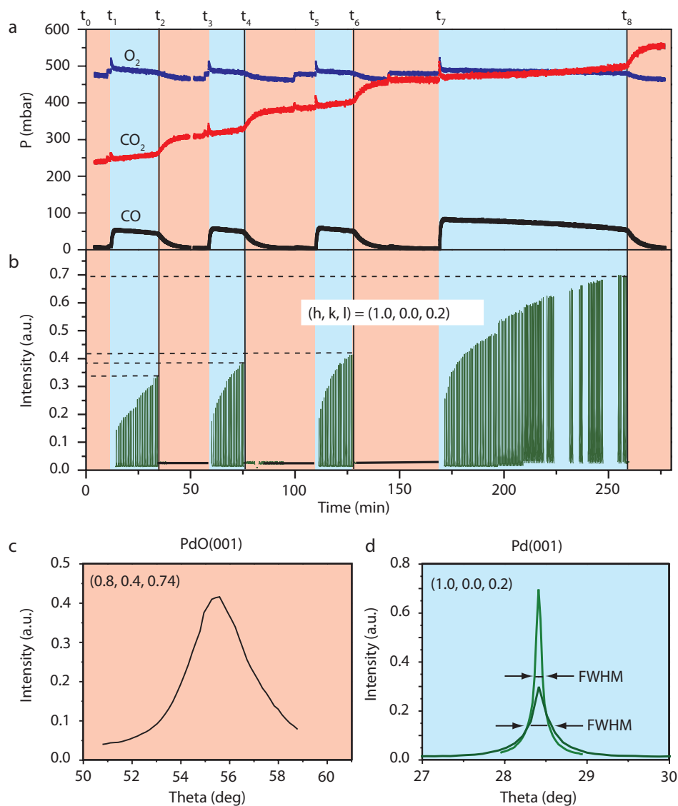
Figure 4.6: Cycles of spontaneous oxidation and forced reduction of the Pd(100) surface during CO oxidation at 460 K in a batch reactor. a ) Partial pressures of the reactants \text{CO} and \text{O}_2 and the reaction product \text{CO}_2 . b ) Series of rocking scans of the Pd(100) surface diffraction peak at (h, k, l) = (1, 0, 0.2) . c ) Rocking scan of the PdO(001) peak of the oxidized palladium surface at (h, k, l) = (0.8, 0.4, 0.74) . d ) Individual rocking scan of the (1, 0, 0.2) crystal truncation rod of Pd(100) from the series in (b).
