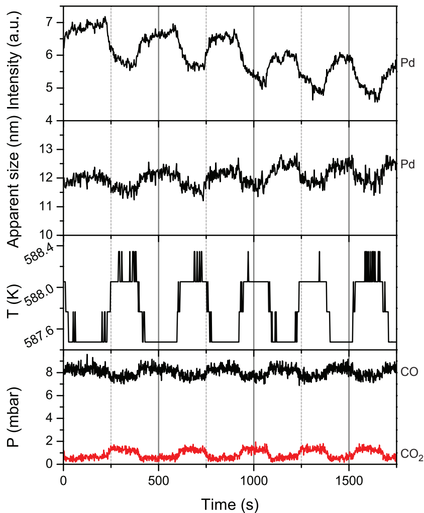
Figure 5.3: Spontaneous oscillations during CO oxidation on the 15 nm diameter Pd particles supported on \text{SiO}_2 . Measurements were performed in a constant flow of a \text{CO/O}_2/\text{Ar} gas mixture with an \text{O}_2 pressure of 210 mbar, an argon pressure of 281 mbar and a CO pressure of 9 mbar flowing at 50 \text{ ml}_n \text{ min}^{-1} . The mass spectrometry signals from CO and \text{CO}_2 show that the reaction rate oscillates (lower panel), which in turn makes the temperature vary (third panel). Note that the temperature variations amount to just a few times the least significant bit of the digitized temperature scale. The top two panels show the diffracted intensity from the Pd particles ( 2\theta = 17.6^\circ ) and the apparent Pd nanocrystal size, derived from the diffraction line widths.
