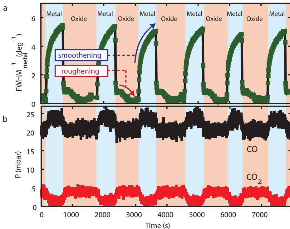
Figure 4.1: Spontaneous oscillations in the CO oxidation rate on Pd(100) as measured by SXRD and mass spectrometry. Measurements were performed at a temperature of 447 K in a constant flow of a \text{CO}/\text{O}_2/\text{Ar} gas mixture with an oxygen pressure of 500 mbar, an argon pressure of 675 mbar and a CO pressure of 25 mbar flowing at 50 \text{ ml}_n \text{ min}^{-1} . a) The \text{FWHM}_{\text{metal}}^{-1} (inversely proportional to the step density and a measure of the smoothness of the surface) of the diffraction peak at (h, k, l) = (1, 0, 2) . b) The partial pressure in the reactor of CO and \text{CO}_2 pressures as measured by mass spectrometry. At high \text{CO} partial pressures P_{\text{CO}} , the diffraction pattern shows that the surface structure is close to a bulk-like truncation of the Pd crystal (the reaction kinetics indicate that this metal surface is covered by a mixture of O atoms and CO molecules). At low P_{\text{CO}} , new diffraction peaks are found that correspond to a thin \text{PdO}(101) layer (e.g. (h, k, l) = (0.8, 0.4, 0.73) see Fig. 4.4). The colors indicate whether the SXRD intensities identify the Pd(100) surface to have a metal structure (light blue) or to be covered by a thin oxide film (light red).
