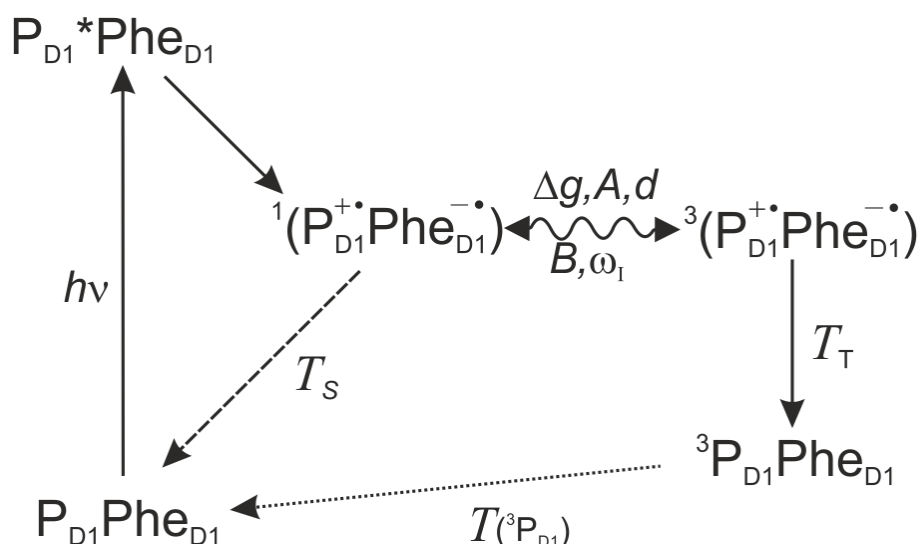
Figure. 5.7: Kinetics and spin dynamics of electron transport for quinone blocked PSII systems and for D1D2 preparations lacking both quinones. Upon removal or double reduction of Q_A the lifetime of the singlet radical pair P_{D1}^{+\bullet}Phe_{D1}^{-\bullet} increases from 20 ns to 250 ns allowing for coherent evolution to the triplet state and photo-CIDNP build-up by the TSM, DD and DR mechanisms.
