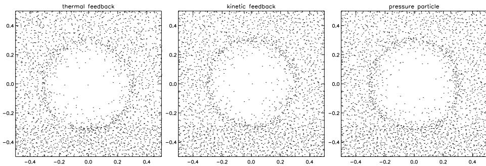
Figure 3.1: Cuts through the particle distribution for the point explosion test. Plotted are the particles closer than 0.05 to the equatorial plane. Each panel shows the results for different feedback method (from left to right: thermal, kinetic and pressure particle feedback).
