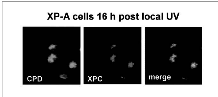
Figure 3. Sustained accumulation of XPC in NER-deficient cells
