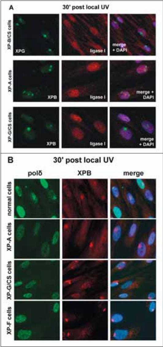
Chapter 10, Figure 2. Differential redistribution of pre- and postincision NER proteins in normal human and XP cells
