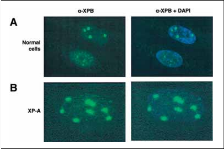
Chapter 6, Figure 5. Reduction of XPB in Unexposed Parts of the Nucleus after Local UV Irradiation
