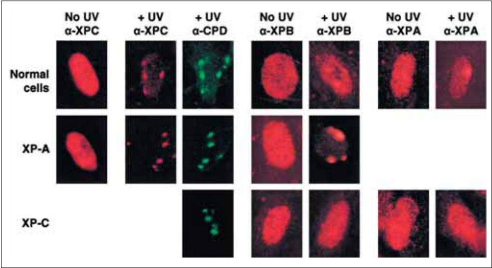
Chapter 6, Figure 4. Recruitment of NER Proteins to Sites of UV Damage
