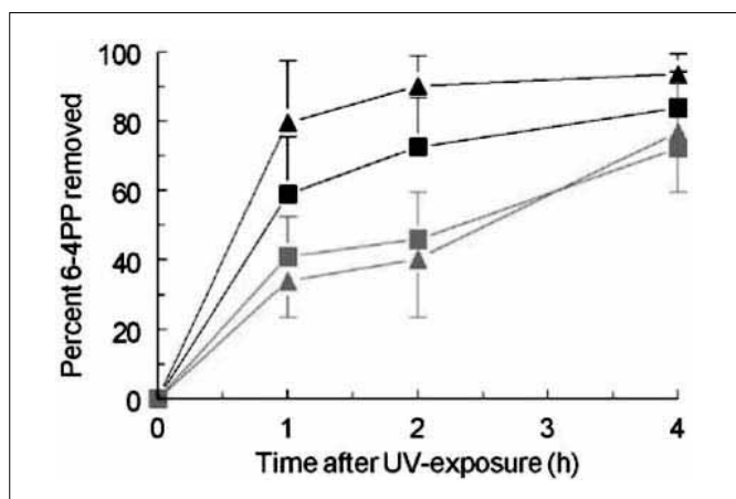
Figure 6. 6-4PP repair in normal human fibroblasts (VH10hTert) and XP-E fibroblasts (GM01389hTert) after local and global UV irradiation with 5 J/m 2 as measured by immunofluorescence
