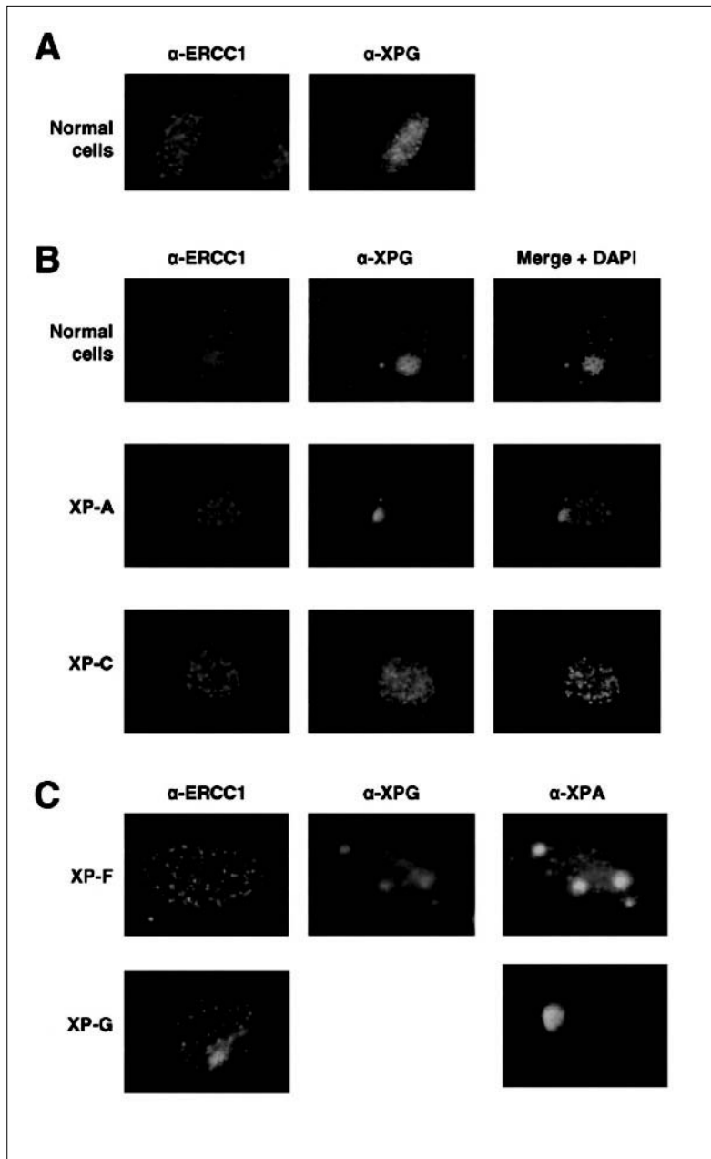
Figure 6. Recruitment of the NER Endonucleases to the Sites of UV Damage Confluent fibroblasts were UV irradiated (30 J/m 2 ) through 3 \mu m filters or mock irradiated, fixed 15 min after UV exposure and immunolabeled for ERCC1, XPG, or XPA. (A) Unexposed normal human fibroblasts (VH25) were immunolabeled for ERCC1 and XPG. (B) Normal human (VH25), XP-A (XP25RO), and XP-C (XP21RO) fibroblasts were immunolabeled for ERCC1 and XPG. (C) XP-F (XP24KY) and XP-G (XPCS1RO) fibroblasts were immunolabeled for XPG and ERCC1, respectively, or XPA. See the Appendix for a colour version of this figure.
