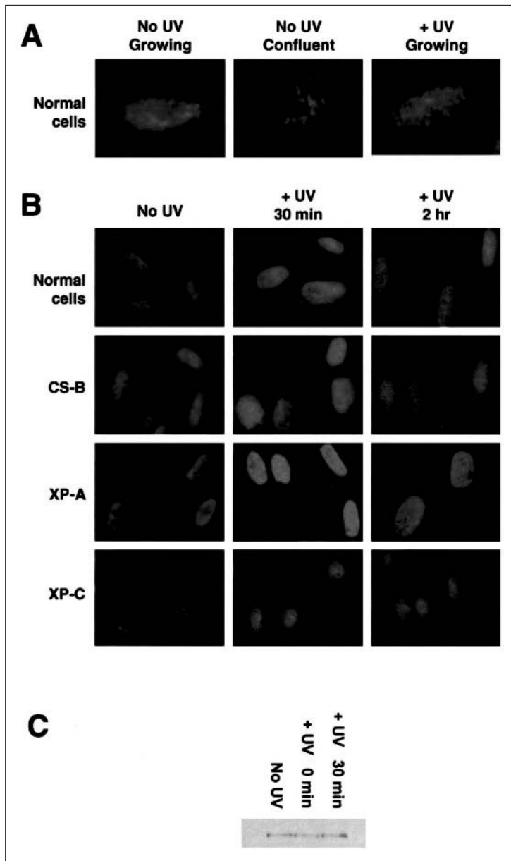
Figure 2. Intensity of the TFIIF Immunofluorescent Signal in Confluent Cells as a Function of Time after UV Exposure
