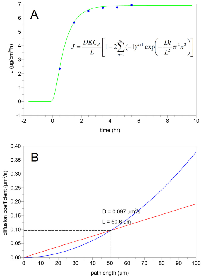
Figure 1: A) Plot of the benzoic acid flux trough a SCS model membrane composed of CER, CHOL and FFA in molar ratios of 1:2:1. The dots denote the measured flux values while the solid line denotes the fit of the diffusion formula (also shown in figure A) with the measured flux values. B) Solutions for D and L from the fit of the diffusion formula with the flux data in (A). The blue line depicts all possible values for D/L resulting from a fit with the steady state part of the flux data and the red line depicts all values for D/L^2 resulting from a fit with the up-going part of the flux data. A unique solution for both D and L is found when the two lines (denoting both fits) coincide. These values are also depicted in figure B.
