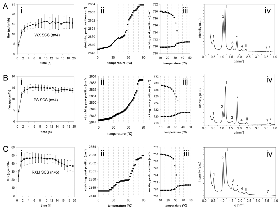
Figure 3: i) Plots of the BA permeation versus time, ii) \text{CH}_2 symmetric stretching frequency as function of temperature, iii) thermotropic response of the FTIR \text{CH}_2 rocking frequencies and iv) the SAXD pattern of A) WX SCS, B) PS SCS and C) RXLI SCS. In the SAXD patterns, the Arabic numbers denote diffraction orders of the LPP, the Roman numbers indicate reflections assigned to the SPP and asterisks mark the reflections of crystalline CHOL. In the figures depicting the \text{CH}_2 rocking vibrations the open squares are calculated with the peak fitting procedure.
