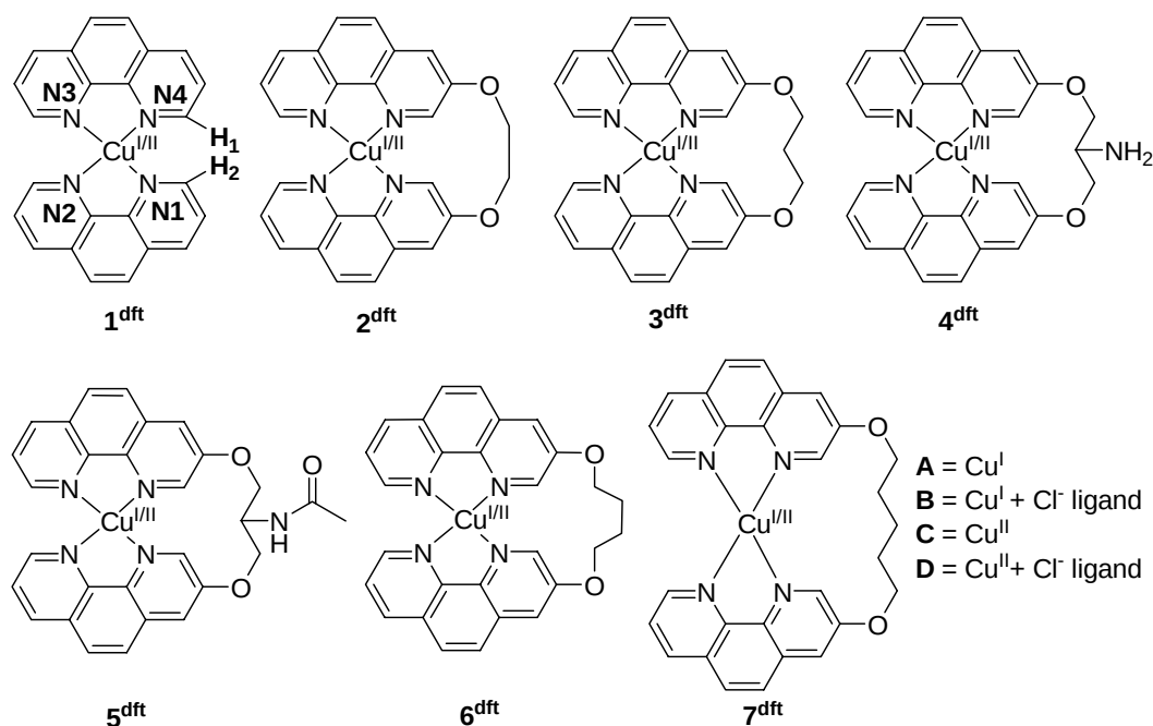
Figure 2.1 The optimized structures of complexes 1^{\text{dft}} [ \text{Cu}^{\text{I/II}}(\text{phen})_2 ], 2^{\text{dft}} \text{Cu}(\text{3-ethyl-Clip-Phen}) , 3^{\text{dft}} \text{Cu}(\text{3-propyl-Clip-Phen}) , 4^{\text{dft}} \text{Cu}(\text{3-Clip-Phen}) , 5^{\text{dft}} \text{Cu}(\text{3-acetyl-Clip-Phen}) , 6^{\text{dft}} \text{Cu}(\text{3-butyl-Clip-Phen}) and 7^{\text{dft}} \text{Cu}(\text{3-pentyl-Clip-Phen}) were calculated for the two oxidation states and with or without chloride as a fifth ligand, namely \text{Cu}^{\text{I}} (A), \text{Cu}^{\text{I}} - \text{Cl}^- (B), \text{Cu}^{\text{II}} (C) and \text{Cu}^{\text{II}} - \text{Cl}^- (D). N.B. The nitrogen atoms closest to the bridges are numbered N1 and N4.
