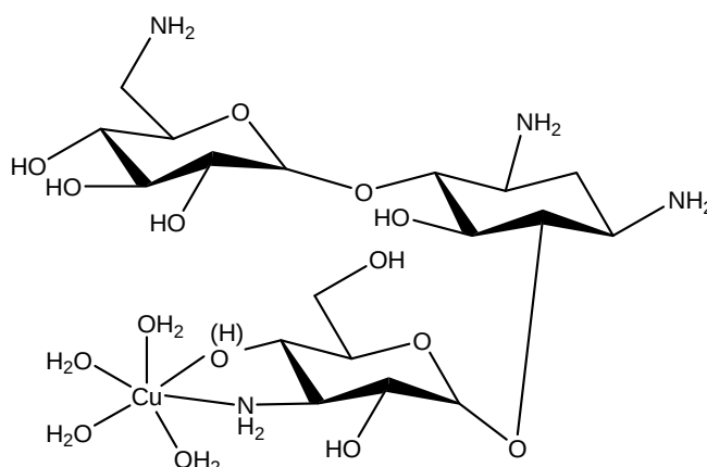
Figure 1.23 Possible structure for \text{Cu}^{\text{II}} (kanamycin). [244]
