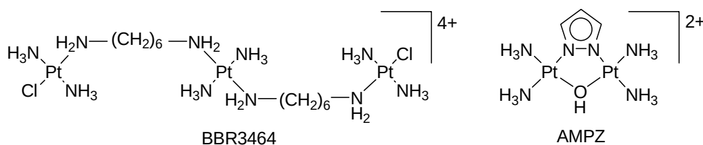
Figure 1.11 Structural formulae of the polynuclear platinum complexes BBR3464 and AMPZ.
