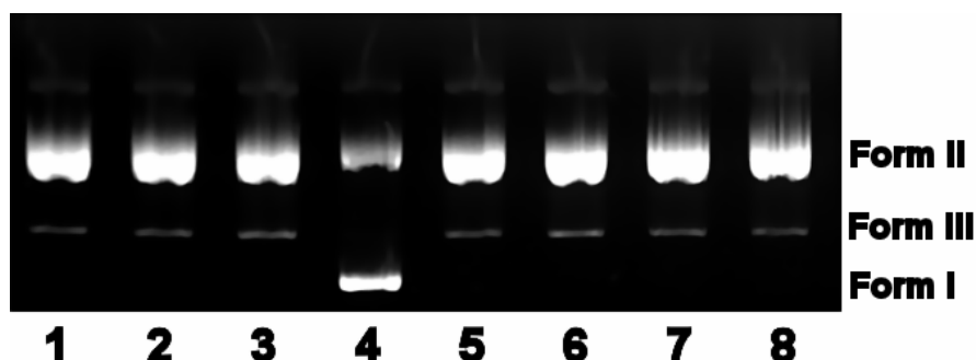
Figure 8.5 Cleavage reactions mediated by [Ru(dtdeg)Cu] in the presence of various scavengers performed in air (except lane 4). All experiments were performed with a complex concentration of 5 \mu M. Lane 1: no extra additives. Lane 2: 100 \mu M NaN 3 . Lane 3: 0.5 units superoxide dismutase. Lane 4: under argon. Lane 5: in the dark. Lane 6: under dioxygen. Lane 7: 20 \mu M DMSO. Lane 8: 20 \mu M ethanol.
