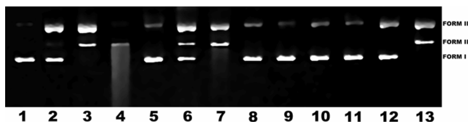
Figure 5.2 Comparative oxidative cleavage experiments of \Phi X174 plasmid DNA for complexes Cu(Asym- cis ) , Cu(Asym- trans ) , Cu(Sym- trans ) and Cu(3-Clip-Phen) in the presence of 5 mM MPA. Lane 1: control DNA. Lane 2: 50 nM Cu(Sym- trans ) . Lane 3: 100 nM Cu(Sym- trans ) . Lane 4: 250 nM Cu(Sym- trans ) . Lane 5: 50 nM Cu(Asym- cis ) . Lane 6: 100 nM Cu(Asym- cis ) . Lane 7: 250 nM Cu(Asym- cis ) . Lane 8: 50 nM Cu(Asym- trans ) . Lane 9: 100 nM Cu(Asym- trans ) . Lane 10: 250 nM Cu(Asym- trans ) . Lane 11: 50 nM Cu(3-Clip-Phen) . Lane 12: 100 nM Cu(3-Clip-Phen) . Lane 13: 250 nM Cu(3-Clip-Phen) .
