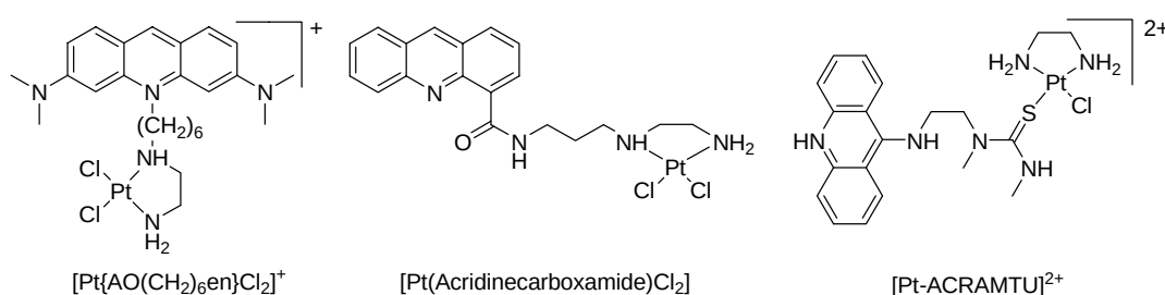
Figure 1.14 Structural formulae of bifunctional platinum complexes including an acridine group.
