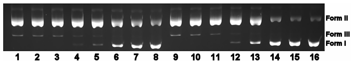
Figure 8.6 Influence of the ionic strength on the cleavage abilities of Cu(terpy) and [Ru(dtdeg)Cu] . Lanes 1-8: Cu(terpy) (5 \mu M). Lanes 9-16: [Ru(dtdeg)Cu] (2 \mu M). Lanes 1
