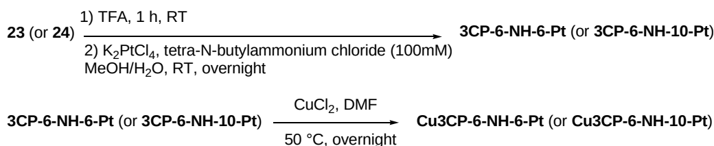
Scheme 6.5 Preparation of the complexes 3CP-6-NH-6-Pt , 3CP-6-NH-10-Pt , Cu3CP-6-NH-6-Pt and Cu3CP-6-NH-10-Pt . 3CP-6-NH-6-Pt and 3CP-6-NH-10-Pt have been characterized by ^1\text{H-NMR} , ^{195}\text{Pt-NMR} , IR, Mass and UV-Vis. Cu3CP-6-NH-6-Pt and Cu3CP-6-NH-10-Pt have been characterized by IR, UV-Vis and EPR.
