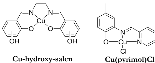
Figure 1.21 Structural formulae of the copper complexes Cu-hydroxy-salen and Cu(pyrinol)Cl complexes. [235, 236]
