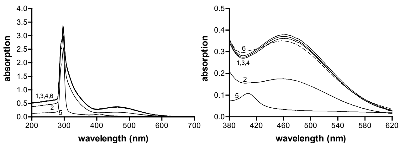
Figure 3: UV-VIS spectra of holo-Tf (10 mg/ml) in the absence (1) or presence of EDTA (1 mM, 2) or TCEP (0.1 or 0.01 mM, lines 3 and 4, respectively) and apo-Tf (10 mg/ml) in the absence (5) or presence (6) of \text{FeCl}_3 and sodium citrate. A typical protein peak is visible around 280 nm (left panel), while only for holo-Tf and apo-Tf incubated for 24 h with \text{Fe}^{3+} a peak around 460 nm is visible (right panel). EDTA is able to scavenge \text{Fe}^{3+} , as is shown by the decrease in absorption at 460 nm, TCEP does not scavenge \text{Fe}^{3+} after 24 h incubation (right panel).
