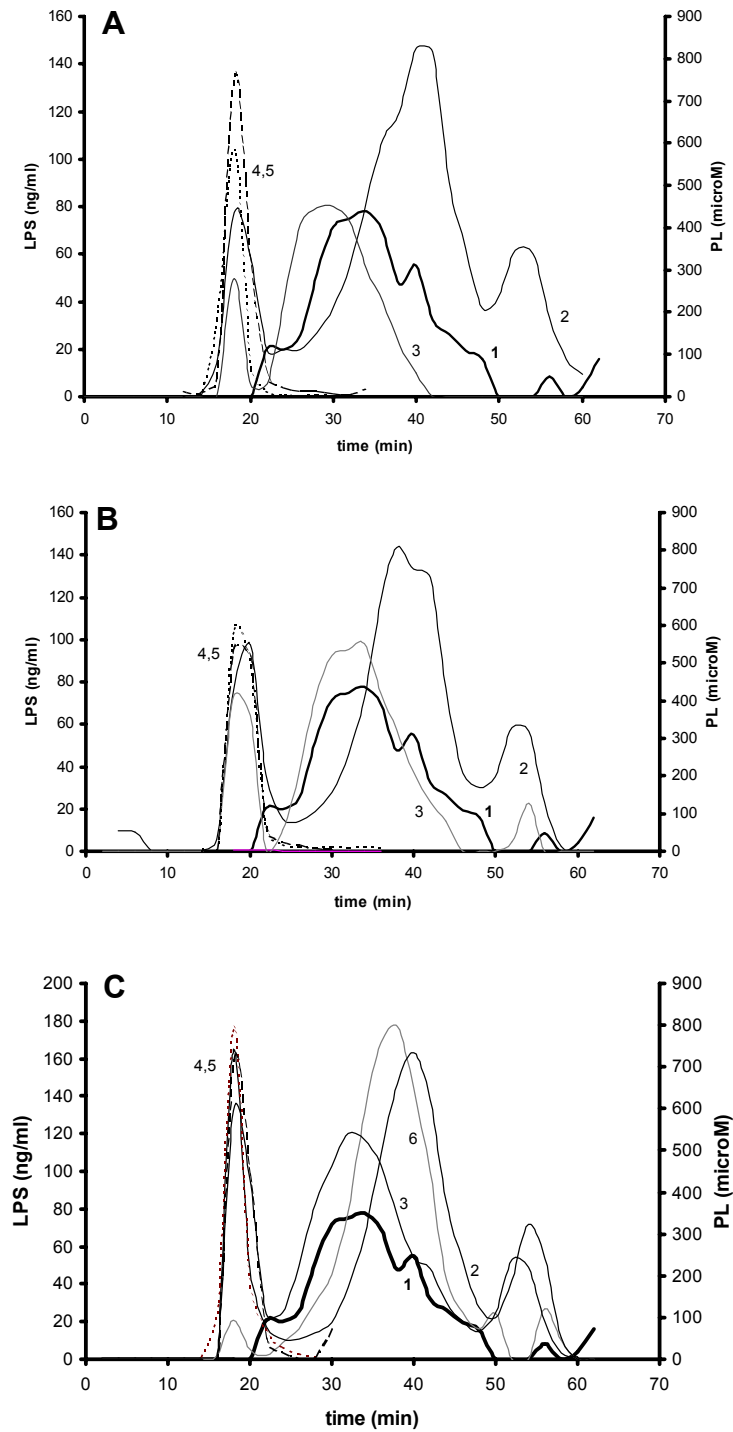
Figure 2: Liposomes of EPC-35 were pre-incubated with fluorescently labelled LPS in the absence or presence of 10 % serum for 2 hours (A), 6 hours (B), or 16 hours (C) before separation on a Sepharose CL4B column. Solid lines is the LPS concentration in ng/ml (left y-axis), dotted lines is the phospholipid (PL) concentration in \mu\text{M} (right y-axis). In each graph lines represent an elution profile of (1) LPS, which is not pre-incubated, (2) LPS + EPC-35 with 10 % serum, (3) LPS + EPC-35 without serum, (4) PL curve of LPS + EPC-35 with 10 % serum, (5) PL curve of LPS + EPC-35 without serum. Figure C also represents an elution profile of LPS pre-incubated with serum (6).
