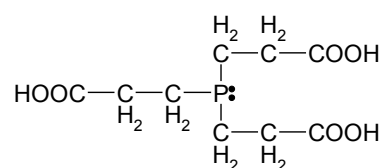
Figure 1: Structure of Tris(2-carboxyethyl)phosphine (TCEP)
