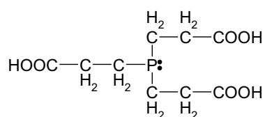
Figure 1: Structure of Tris(2-carboxyethyl)phosphine (TCEP)
