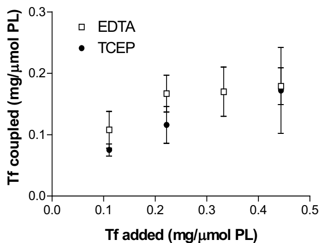
Figure 4: The amount of coupled Tf per \mu\text{mol} phospholipid (PL) is plotted against the added amount of Tf per \mu\text{mol} PL. This shows that the coupling of Tf is saturable at amounts higher than 0.25 mg Tf per \mu\text{mol} PL. The amount of coupling is not changed in the presence of TCEP (0.01 mM) compared to EDTA (1 mM).
