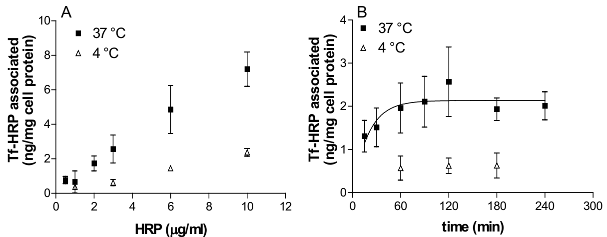
Figure 1: Concentration (A) and time (B) dependent association and binding of Tf-HRP. Incubation of BCEC with Tf-HRP (0.5 – 10 \mu\text{g/ml} ) for 2 h at 37 °C or at 4 °C showed a concentration dependent association of Tf-HRP, which is linear up to 10 \mu\text{g/ml} . The association at 37 °C was approximately 4-fold higher at each concentration tested. Incubation of BCEC with 3 \mu\text{g/ml} Tf-HRP for 15 – 240 minutes at 37 °C or at 4 °C, showed that after approximately 60 minutes equilibrium was reached for the association (determined at 37 °C). Binding was around 4-fold lower at 60, 120 and 180 min. Data represented (mean \pm SD; n = 3 experiments, each performed in quadruplicate) are the specific association (total association corrected for non-specific association); non-specific association was approximately 40% of total association (independent of the concentration).
