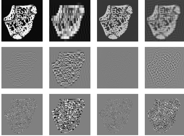
Figure 3.5: Illustrations of the key concepts for Phantom 3; From left to right: 8x8 window, regular; 32x32 window, regular; 8x8 window, random; 32x32 window, random; From top to bottom: central reconstruction; difference between the central reconstruction and the phantom; difference between the rounded central reconstruction and the phantom.
