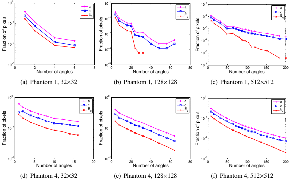
Figure 2.8: Strip model: computed bounds as a function of the number of projection directions for Phantoms 1 and 4.
