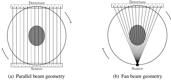
Figure 6.2: Tomography geometry
