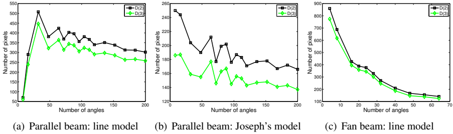
Figure 6.6: Absolute difference between the bound for the number of ones in any binary solution and the number of ones of the phantom.
