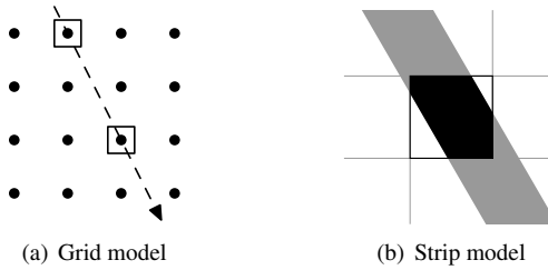
Figure 2.1: Two different projection models.
