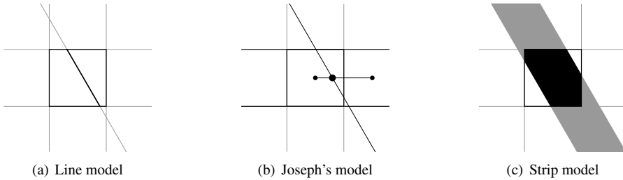
Figure 6.3: Projection models
