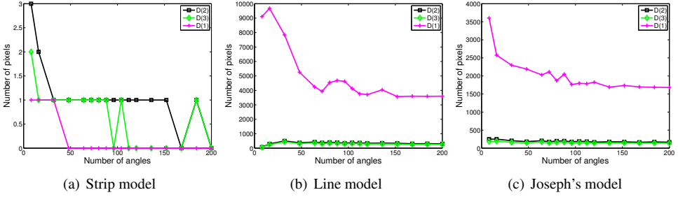
Figure 6.5: Absolute difference between the bound for the number of ones in any binary solution and the number of ones in the phantom.
