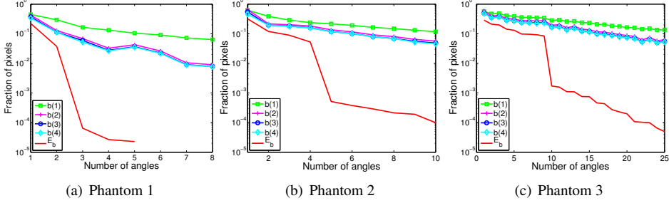
Figure 2.5: Error bounds for DART reconstruction of the three phantoms (size 512 \times 512 ) as function of the number of projection angles. Note that the graphs for b(2) , b(3) , and b(4) have strong overlap and can hardly be distinguished.
