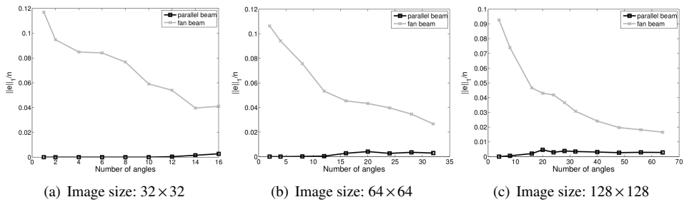
Figure 6.4: Relative \ell_1 -norm of the correction vector \mathbf{e} for the line model in parallel and fan beam tomography.
