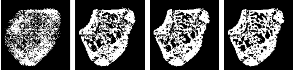
(b) Phantom 7.5(b). Alg. 7.1 with \tau = \frac{1}{\sqrt{128}} . N. proj. angles: left: 4; mid-left: 16; mid-right: 20; right: 24.
