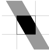
Figure 7.6: The contribution weight of each pixel to each projection component is given by the intersection area between the pixel and the respective strip.
