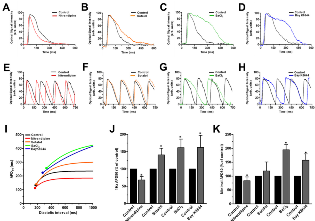
Figure 3. Typical optical action potential records in control (black) and (A) nitrendipine (red), (B) sotalol (orange), (C) BaCl 2 (green) and (D) BayK8644 (blue) treated cultures illustrating treatment effects on 1 Hz APD and minimal APD (E-H) and (I) APD restitution. Colored circles indicate the average minimal APD. Quantification of (J) 1 Hz APD and (K) minimal APD before and after treatments. *: P < 0.05 vs. control.
