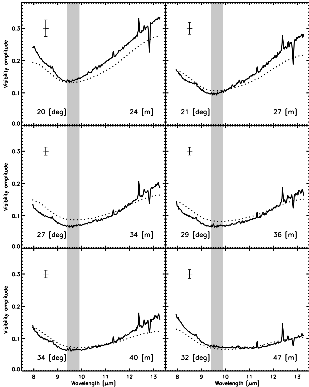
Figure 3.6 — Each panel displays the calibrated visibility amplitude of MWC 349A as function of wavelength for one observed (u, v) point. The position angles and projected length of the employed baselines are indicated in the lower left and right corners of each panel. Also indicated is the uncertainty for each measurement, derived from the scatter of the calibrators in that night. The gray areas indicate wavelength regions at which ozone in the Earth’s atmosphere strongly influences the observed visibilities. The amplitudes measured in these wavelength regions are not included in our analysis. The dashed lines represent visibilities for our best model (see Section 3.3.1).
