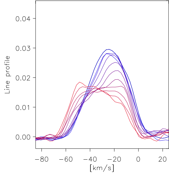
Figure 4.3 — The same as Fig. 4.2 but for the secondary eclipse. One can see BFs of the eleven observations obtained during the secondary eclipse with the line profile of the primary subtracted. The change in radial-velocity during the secondary eclipse is smaller than during the primary eclipse, also the coverage of the secondary is less than the coverage of the primary during its eclipse. This is due to the orbital inclination not being 90^\circ , and the greater distance between the two stars along the line of sight during secondary eclipse (See Fig. 4.5).
