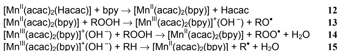
Scheme 3.3: Proposed sets of reactions for each of the catalyst systems.
