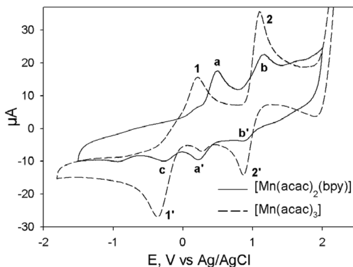
Figure 3.8: Cyclic voltammograms of [Mn(acac) 3 ] and [Mn(acac) 2 (bpy)] in CH 3 CN, [tBu 4 N](PF 6 ) as electrolyte, scan rate 200mV/s. Selected potentials: 1/1' 0.222/-0.373 V; a/a' 0.50/0.203 V; 2/2' 1.111/0.862 V; b/b' 1.165/0.891 V; c -0.28 V.
