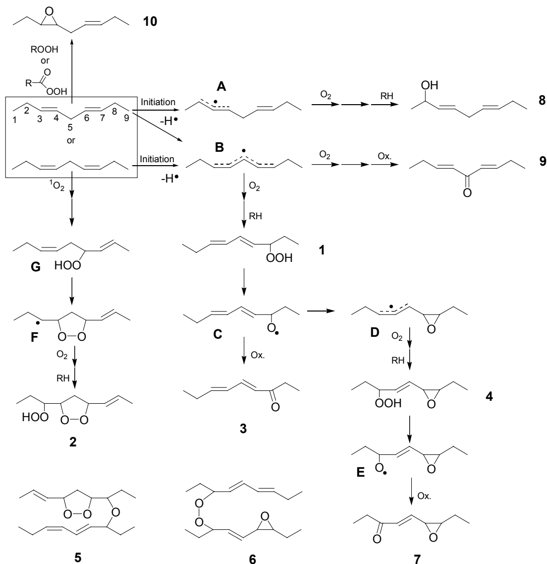
Scheme 1.6: Products of the cobalt-catalysed autoxidation of (E,E) or (Z,Z) -3,6-nonadiene. Products 1-10 were isolated and characterised with ^1H - and ^{13}C -NMR. Species A-F are proposed reaction intermediates. The monomeric products found with the (Z,Z) -isomer were also isolated starting from (E,E) -3,6-nonadiene. [57]
