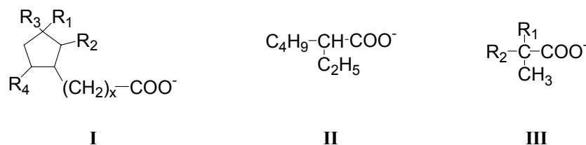
Figure 1.6: Carboxylates used in traditional drier metal soaps. I: Naphthenoate derivative, \text{R}_1 , \text{R}_2 , \text{R}_3 and \text{R}_4 are short alkyl chains or hydrogens. II: 2-ethylhexanoate, often referred to as “octoate”. III: Versetate, typically neodecanoate: \text{R}_1 and \text{R}_2 are alkyl groups and the total number of carbon atoms is ten.
