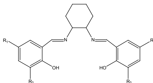
Figure 1.11: Examples of salen type ligands used with manganese as alkyd paint driers. Substituents are \text{R}_1=\text{R}_2=\text{tert-butyl} , or \text{R}_1 = a dodecyl chain, \text{R}_2 = \text{H} .
