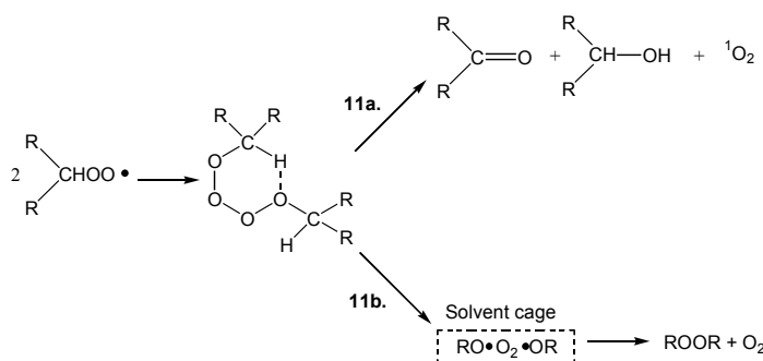
Scheme 1.2: Bimolecular peroxy radical termination via a tetraoxide intermediate. In reaction 11a (the Russel mechanism) an alcohol, ketone and singlet oxygen are formed. In reaction 11' , the tetraoxide intermediate decomposes to yield two alkoxy radicals, which recombine in the solvent cage to form a peroxide cross-link.
