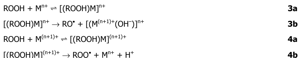
Scheme 1.3: Metal–hydroperoxide complex formation in media of low polarity
