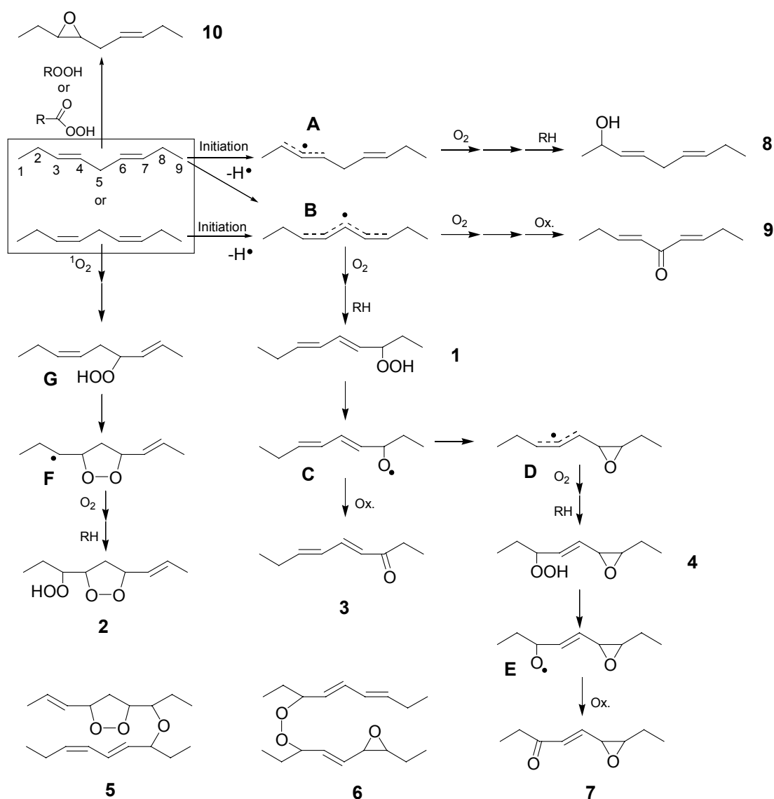
Scheme 1.6: Products of the cobalt-catalysed autoxidation of ( E,E ) or ( Z,Z )-3,6-nonadiene. Products 1-10 were isolated and characterised with 1 H- and 13 C-NMR. Species A-F are proposed reaction intermediates. The monomeric products found with the ( Z,Z )-isomer were also isolated starting from ( E,E )-3,6-nonadiene. [57]
